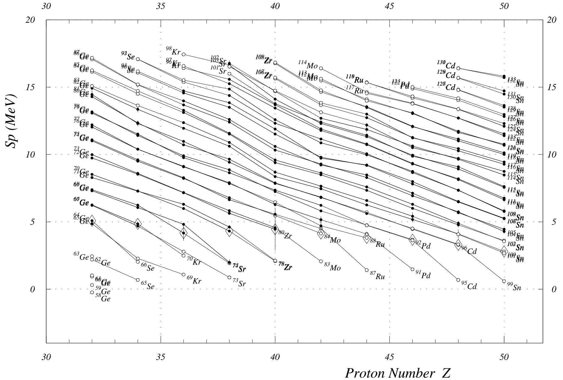
Fig. 3. One-Proton Sep. Energies (even Z) Z = 32 to 50
