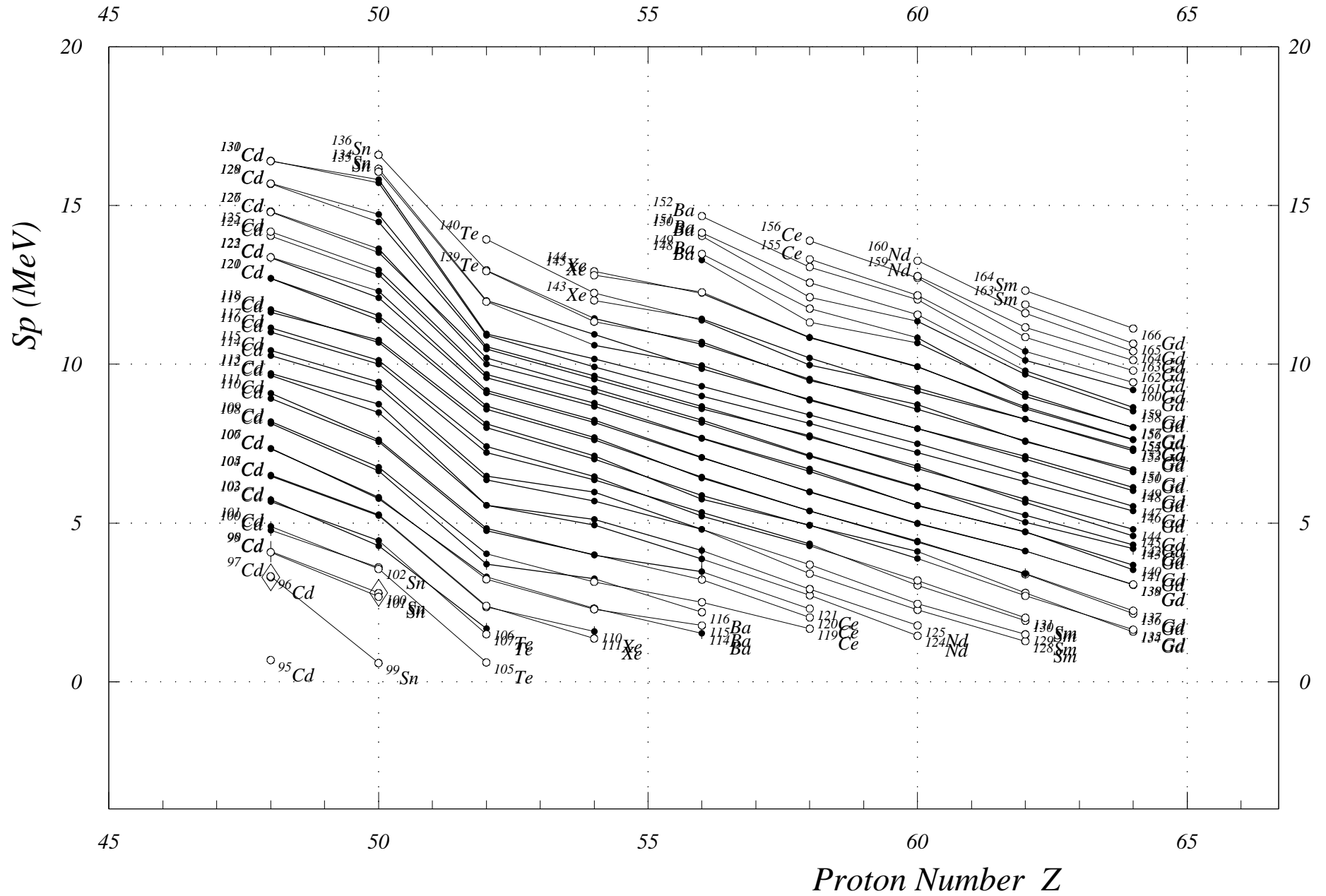
Fig. 4. One-Proton Sep. Energies (even Z) Z = 47 to 65
