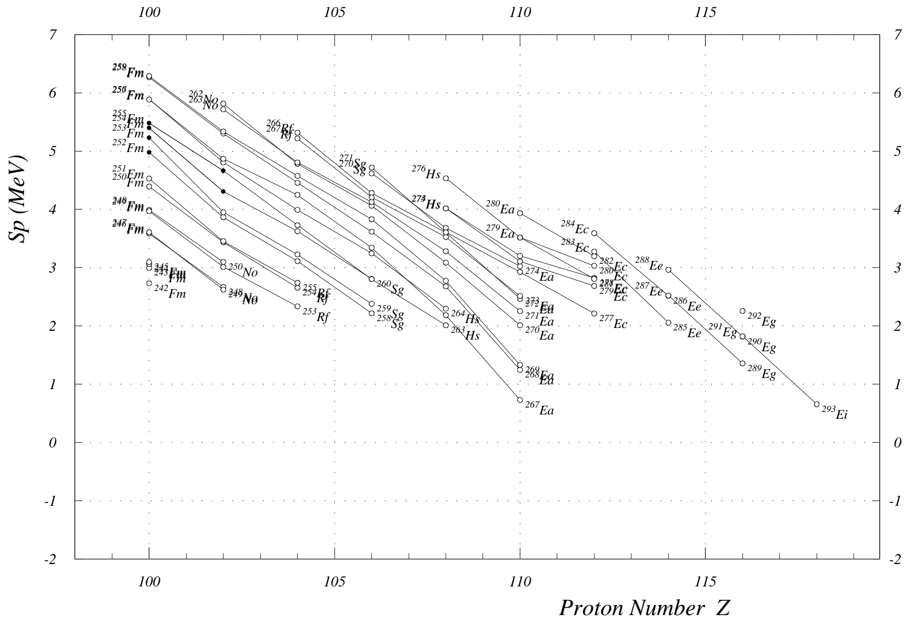
Fig. 8. One-Proton Sep. Energies (even Z) Z = 100 to 118
