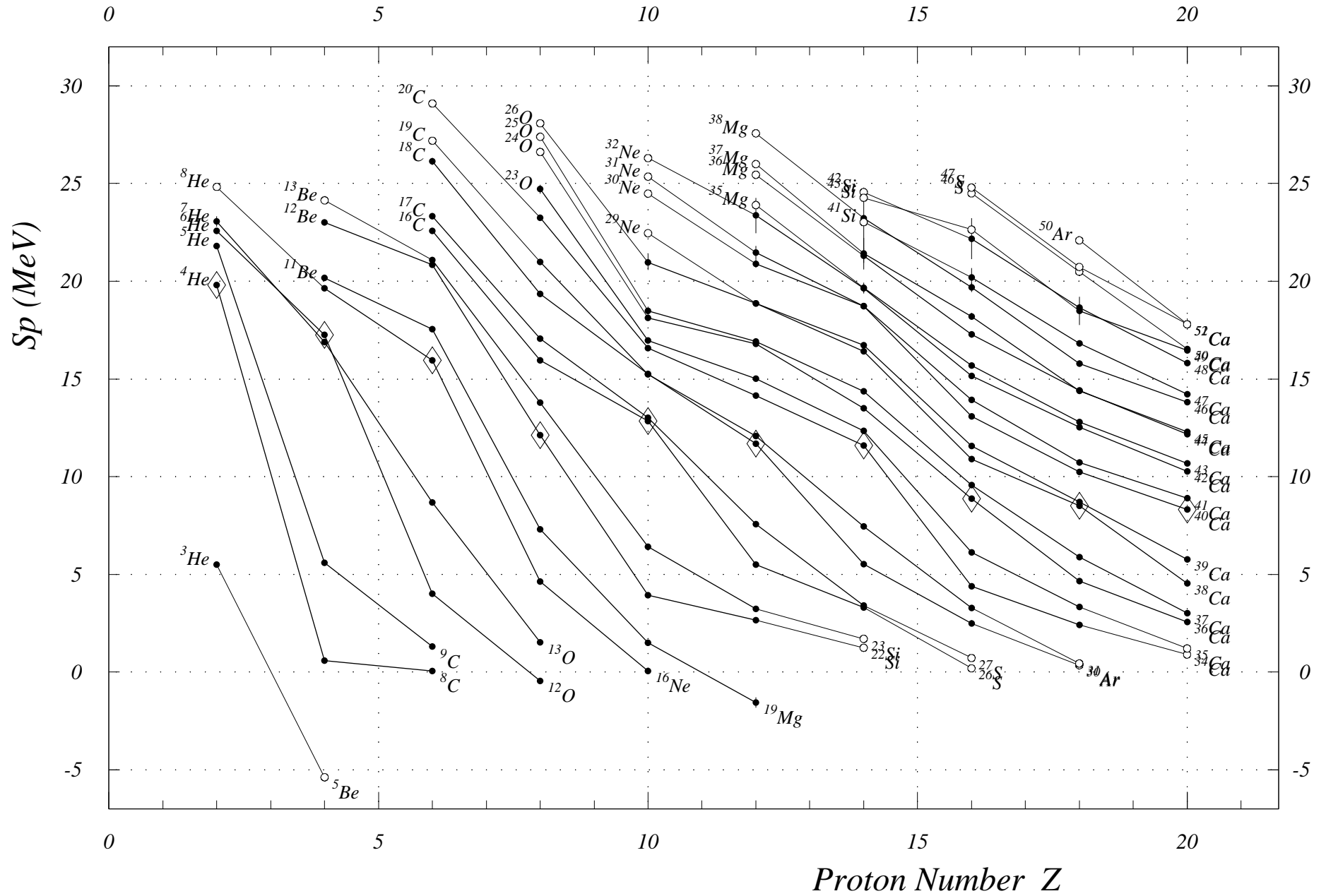
Fig. 1. One-Proton Sep. Energies (even Z) Z = 0 to 20
