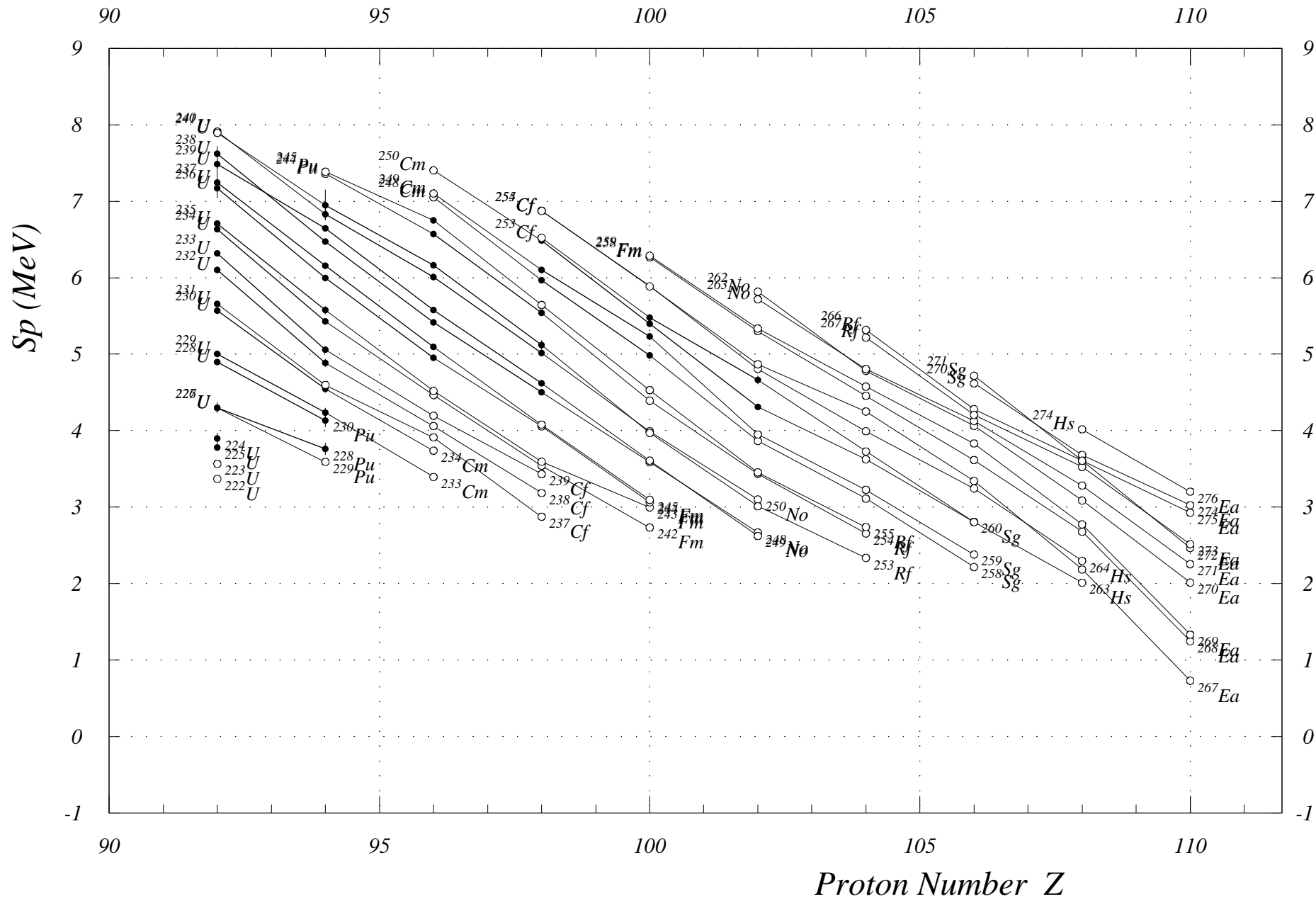
Fig. 7. One-Proton Sep. Energies (even Z) Z = 92 to 110
