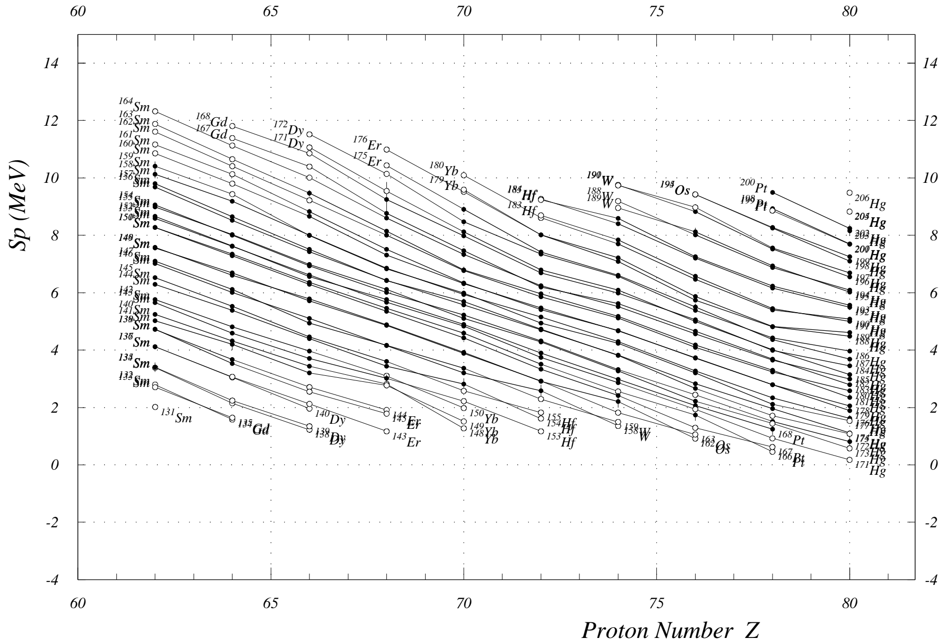
Fig. 5. One-Proton Sep. Energies (even Z) Z = 62 to 80
