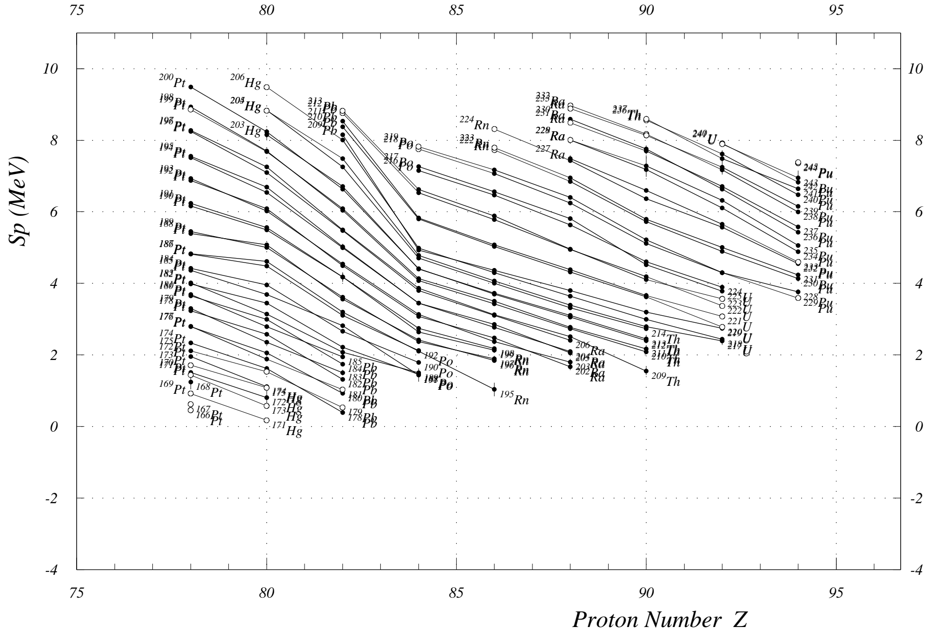
Fig. 6. One-Proton Sep. Energies (even Z) Z = 77 to 95
