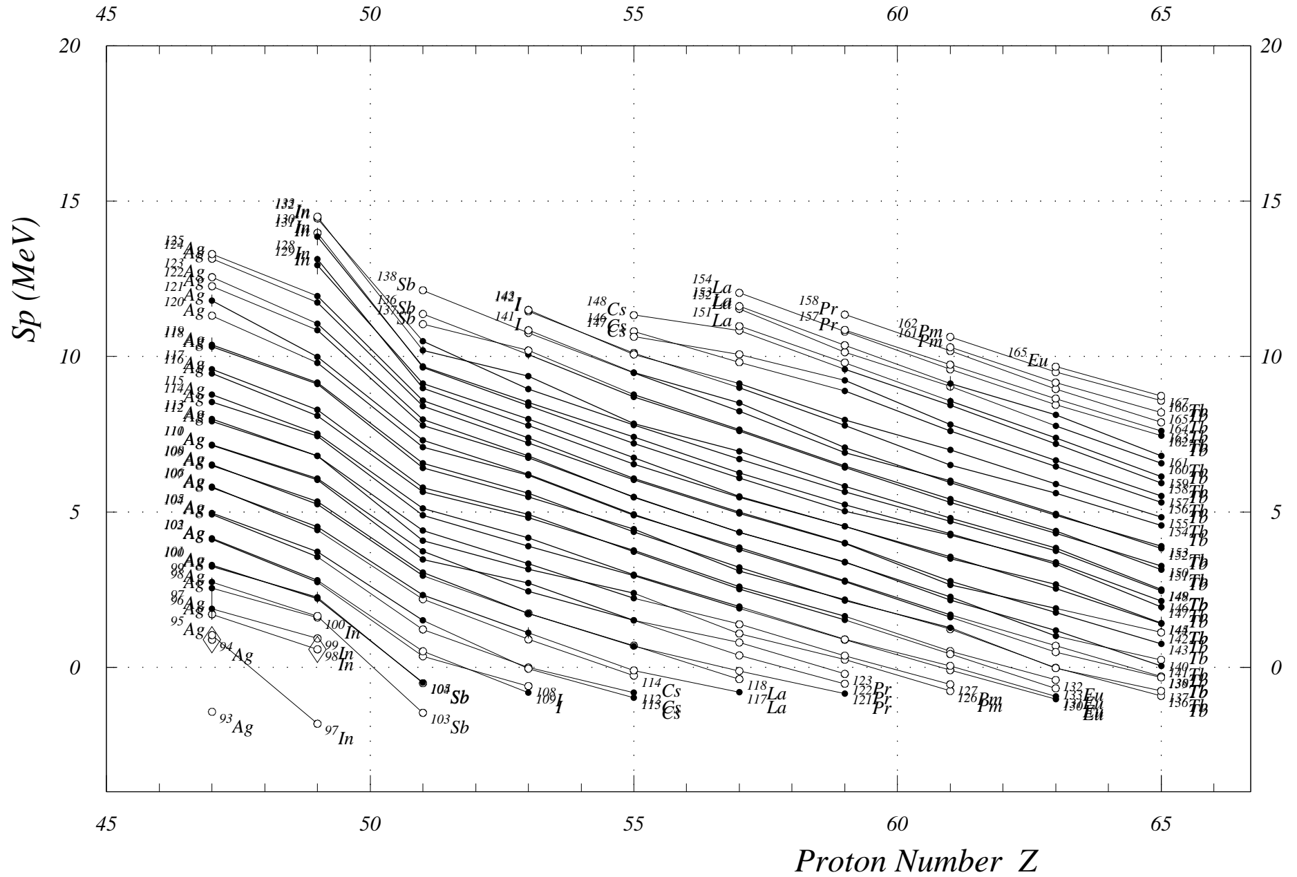
Fig. 4. One-Proton Sep. Energies (odd Z) Z = 47 to 65
