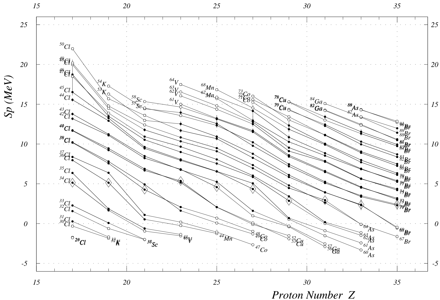
Fig. 2. One-Proton Sep. Energies (odd Z) Z = 17 to 35
