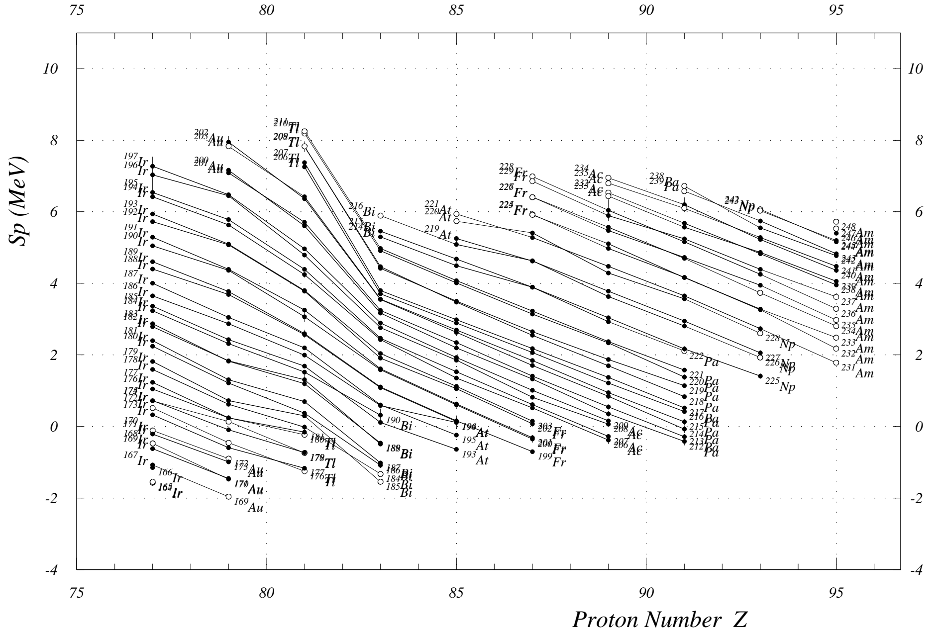
Fig. 6. One-Proton Sep. Energies (odd Z) Z = 77 to 95
