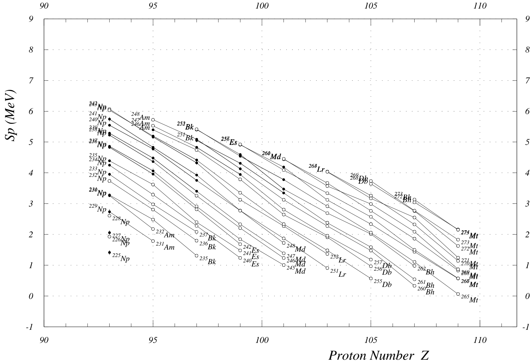
Fig. 7. One-Proton Sep. Energies (odd Z) Z = 92 to 110
