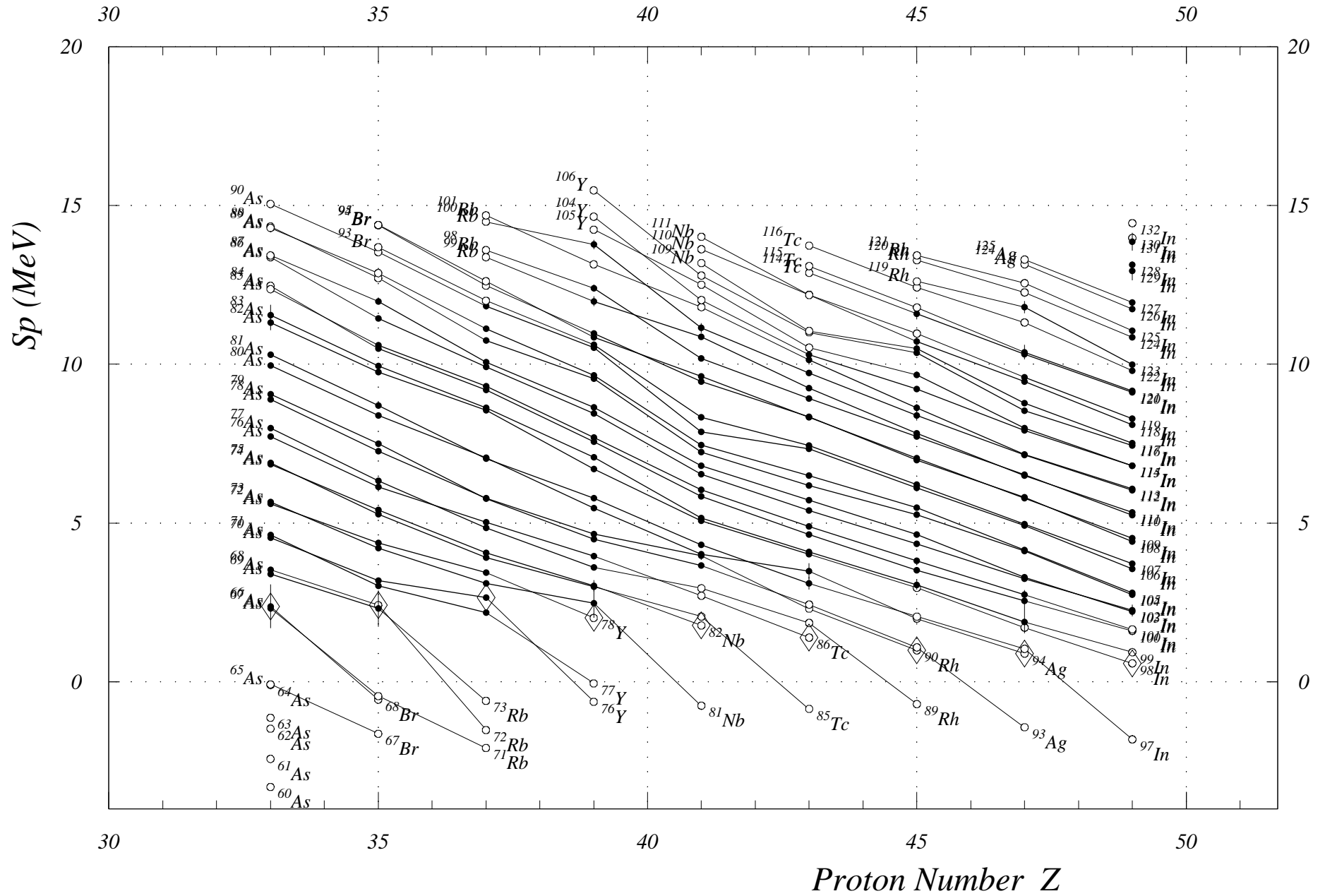
Fig. 3. One-Proton Sep. Energies (odd Z) Z = 32 to 50
