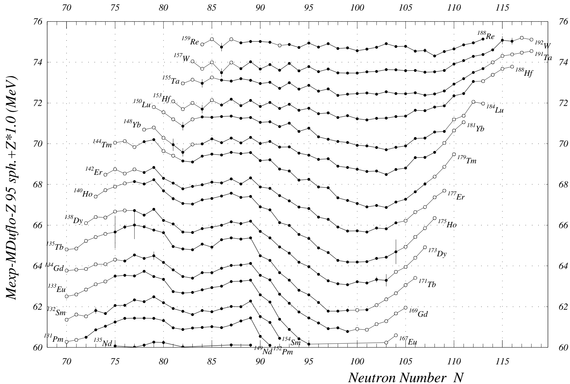
Fig. 6. Mass Exp-Mass Duflo-Z 95 sph. N= 70 to 118
