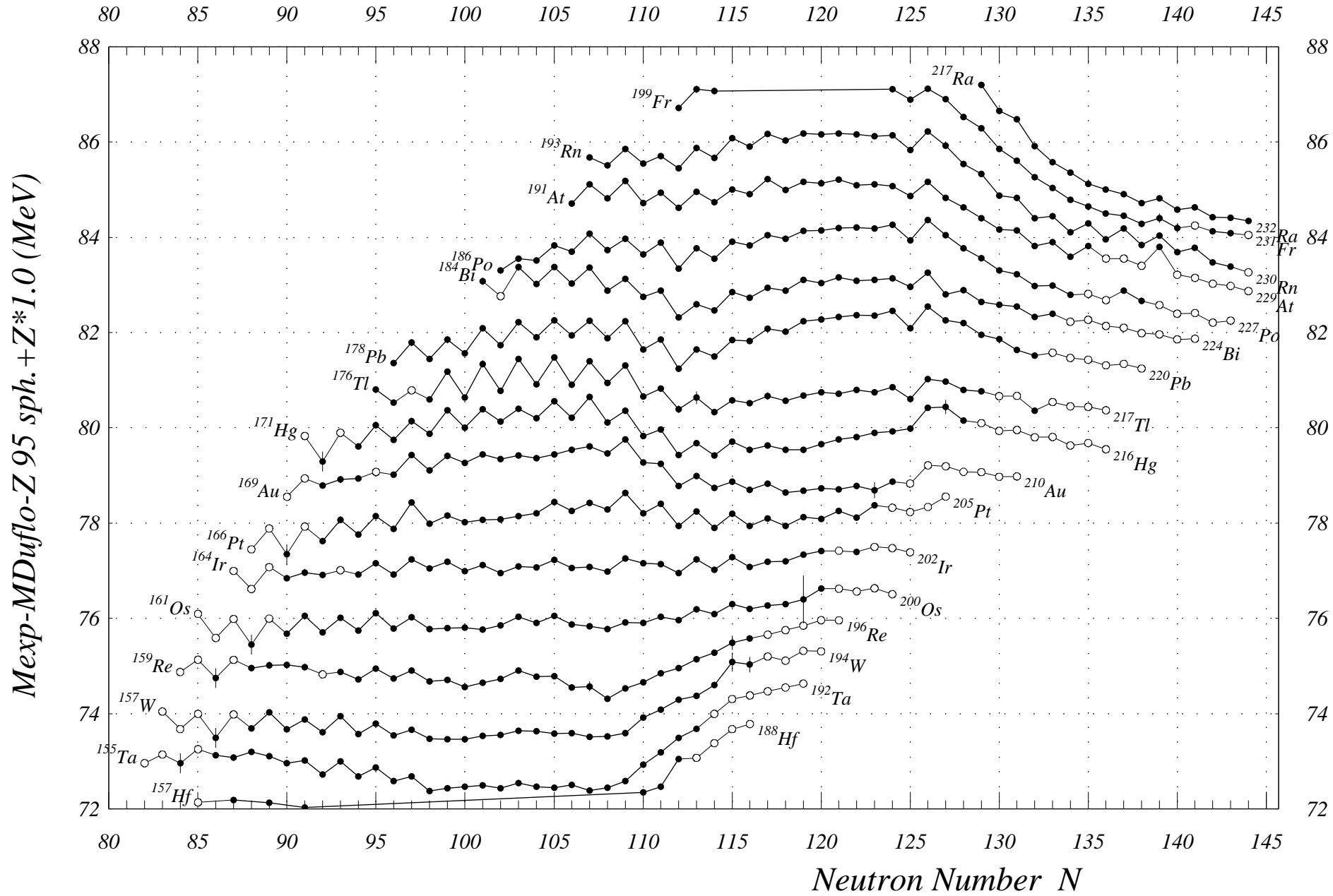
Fig. 7. Mass Exp-Mass Duflo-Z 95 sph. N= 82 to 144
