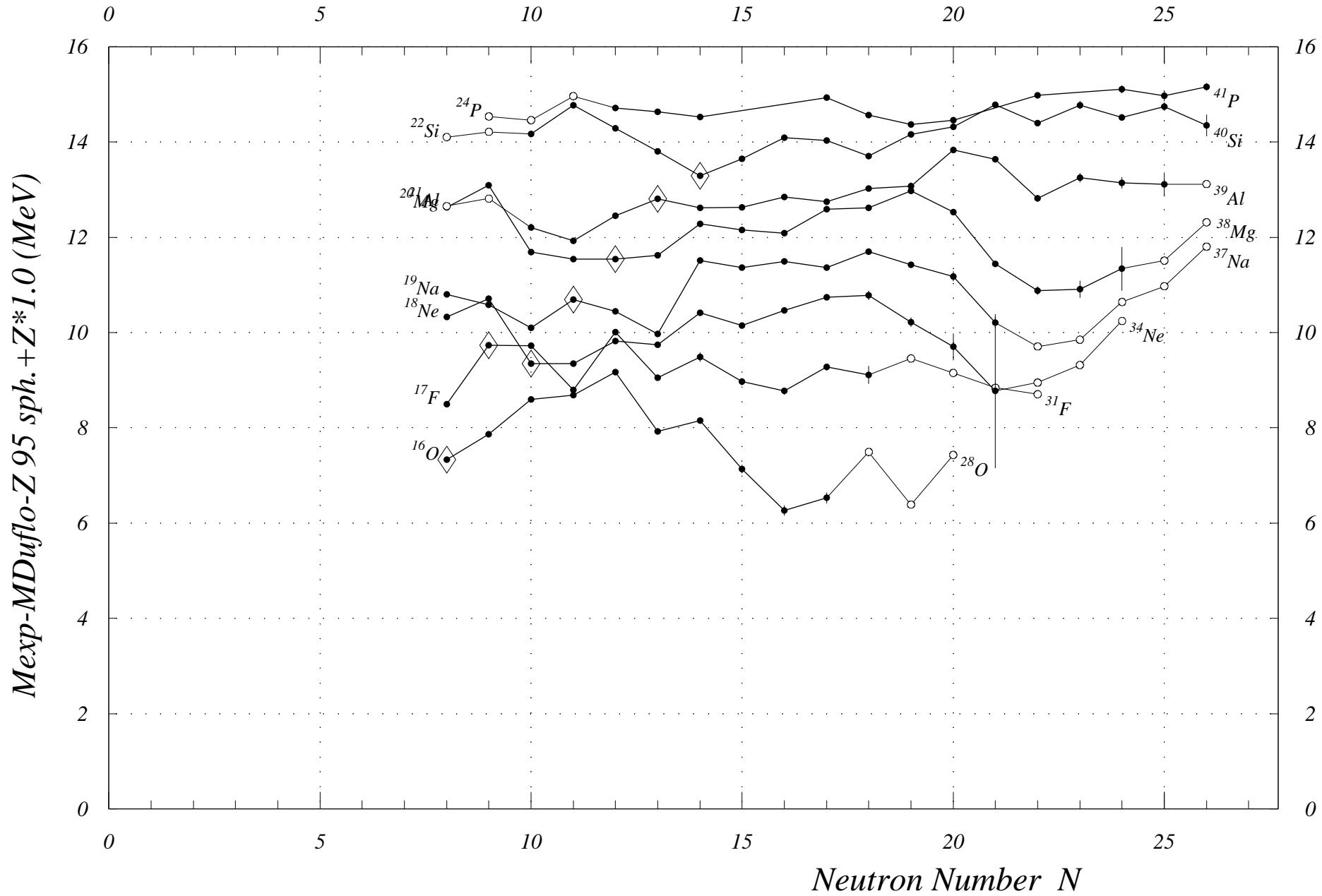
Fig. 1. Mass Exp-Mass Duflo-Z 95 sph. N= 0 to 26
