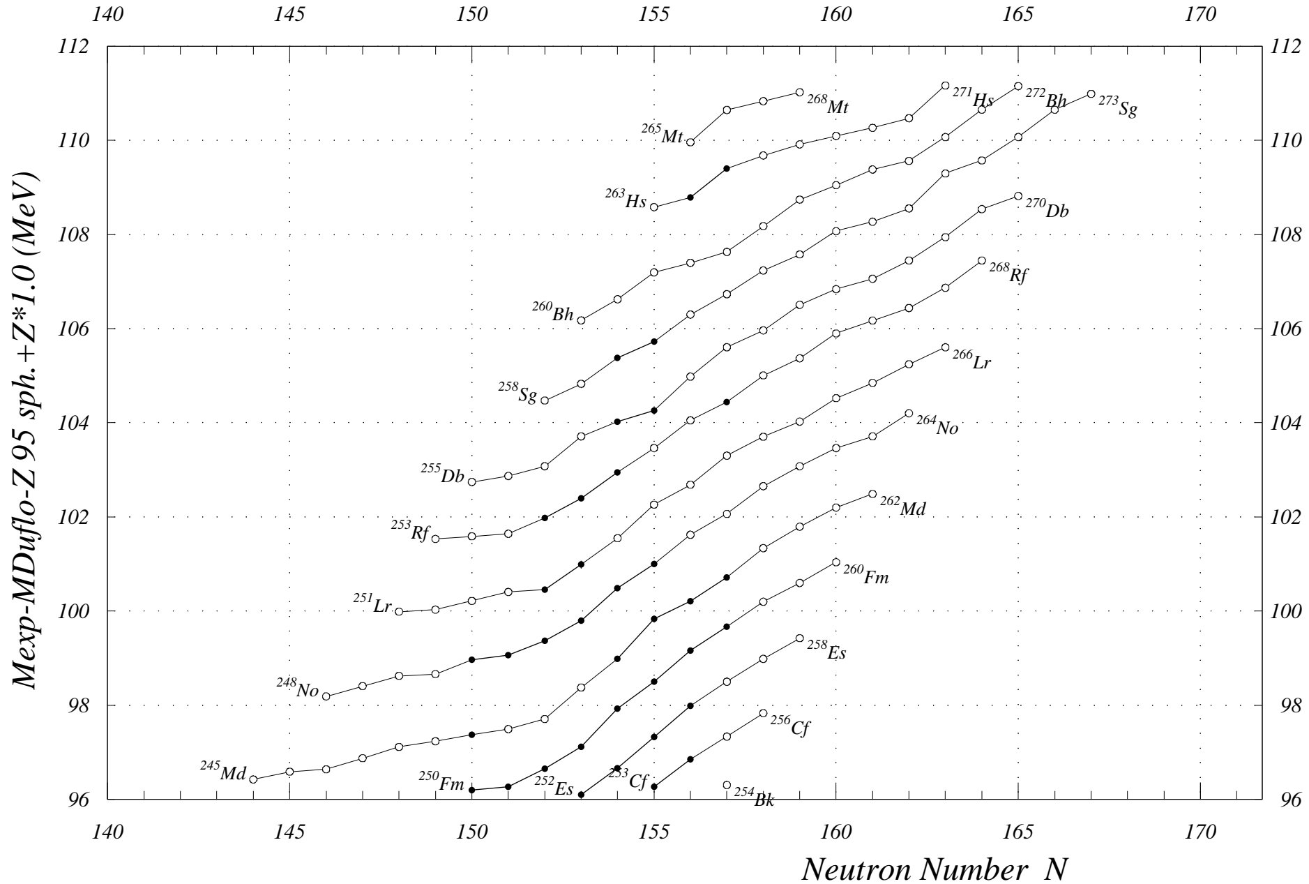
Fig. 9. Mass Exp-Mass Duflo-Z 95 sph. N= 142 to 170
