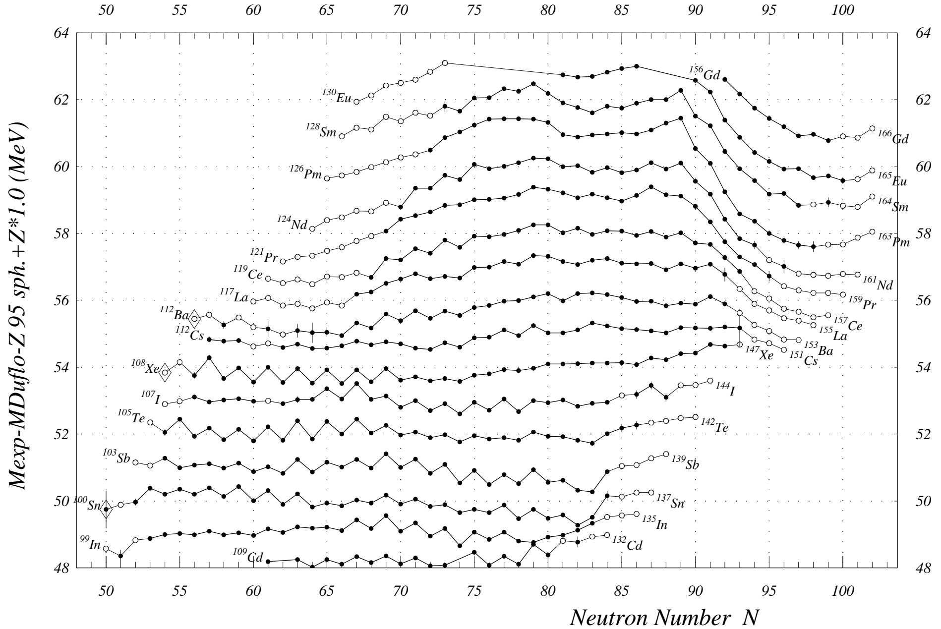
Fig. 5. Mass Exp-Mass Duflo-Z 95 sph. N= 50 to 102
