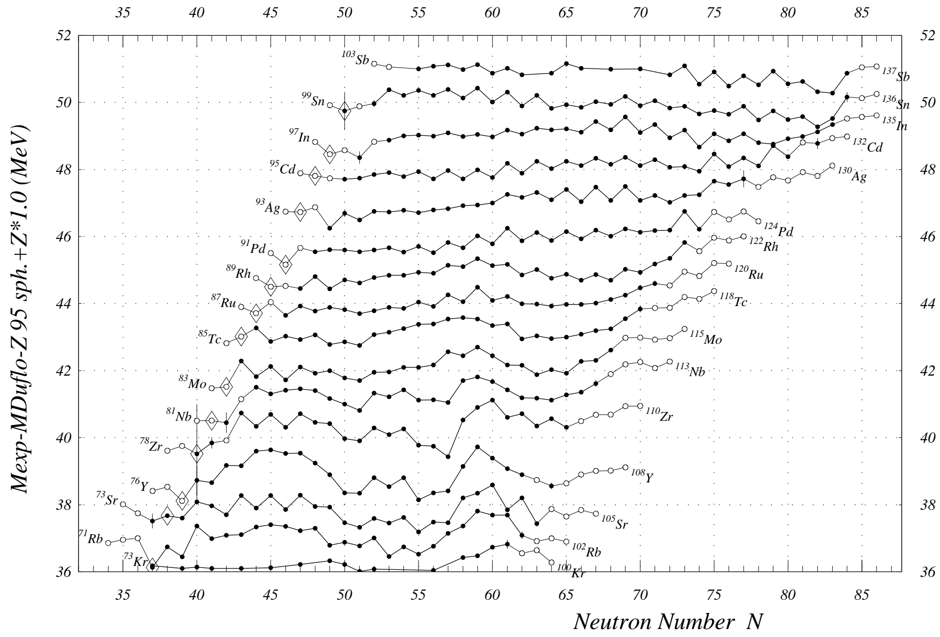
Fig. 4. Mass Exp-Mass Duflo-Z 95 sph. N= 34 to 86
