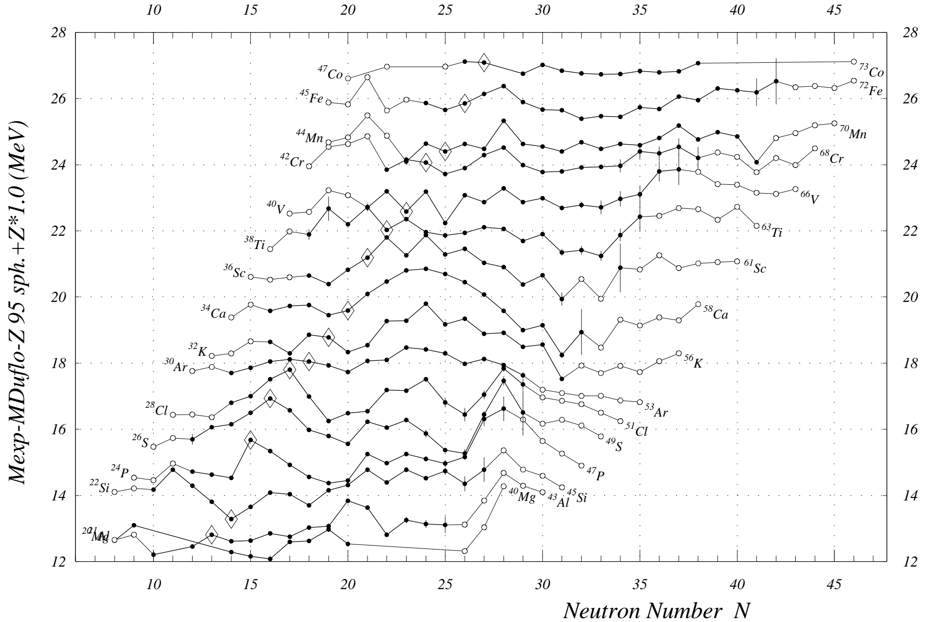
Fig. 2. Mass Exp-Mass Duflo-Z 95 sph. N= 8 to 46
