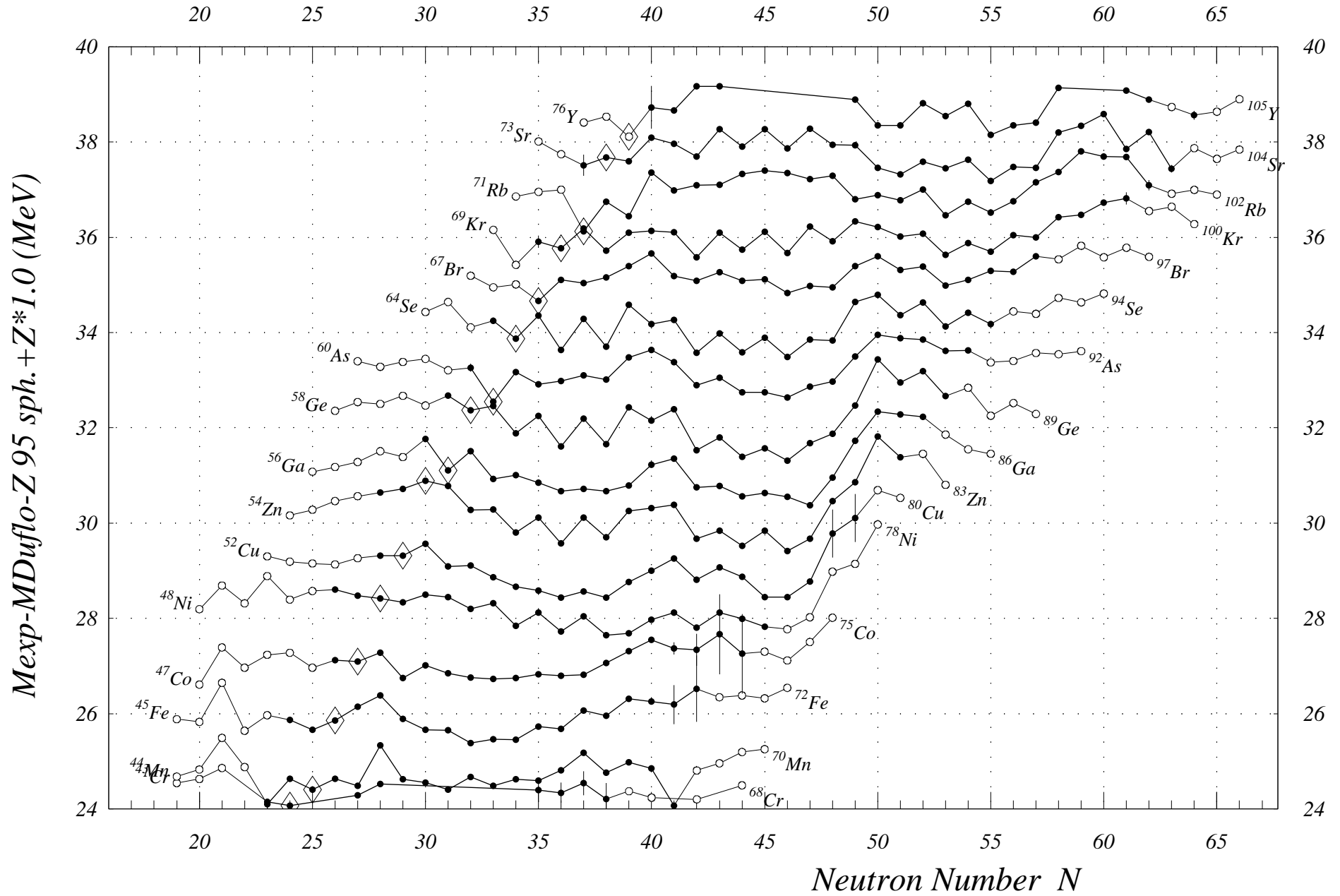
Fig. 3. Mass Exp-Mass Duflo-Z 95 sph. N= 18 to 66
