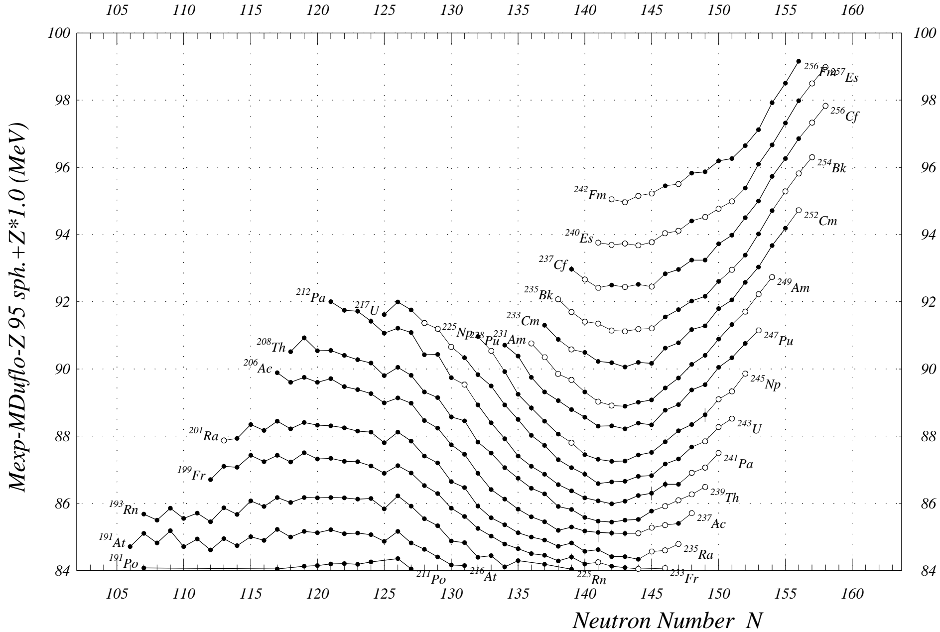
Fig. 8. Mass Exp-Mass Duflo-Z 95 sph. N= 104 to 162
