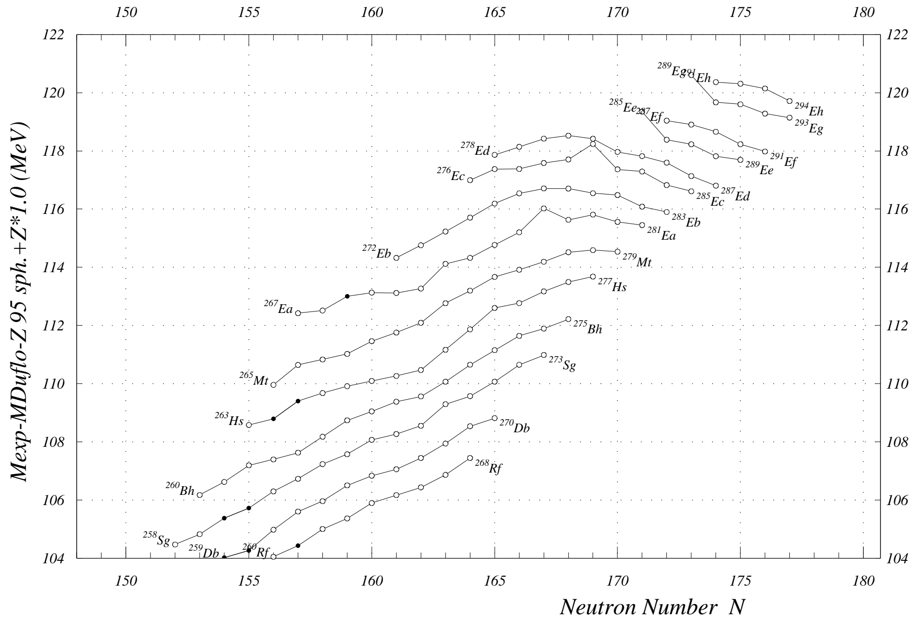
Fig. 10. Mass Exp-Mass Duflo-Z 95 sph. N= 150 to 179
