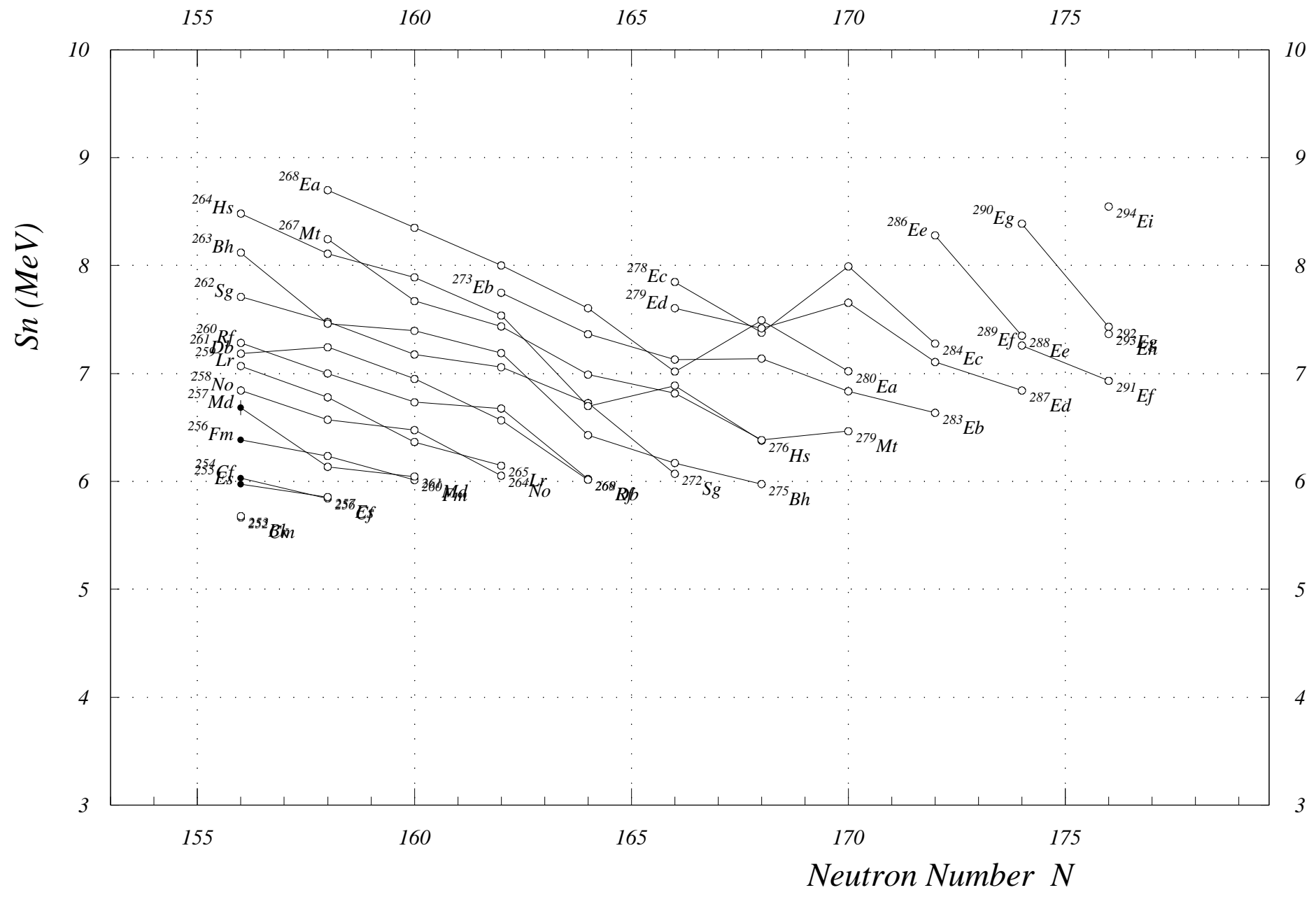
Fig. 9. One-neutron Sep.Energies (even N) N = 155 to 178
