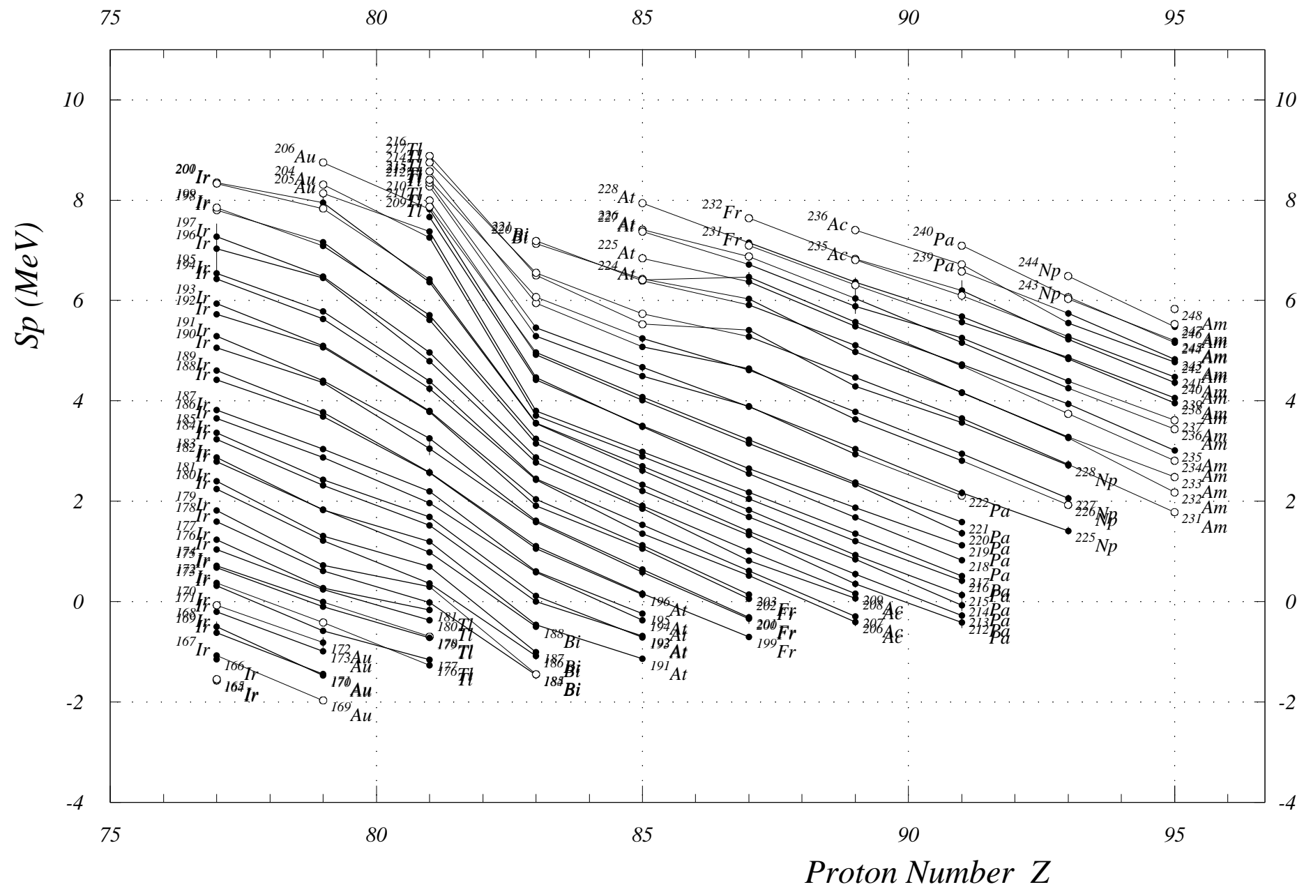
Fig. 15. One-Proton Sep. Energies (odd Z) Z = 77 to 95
