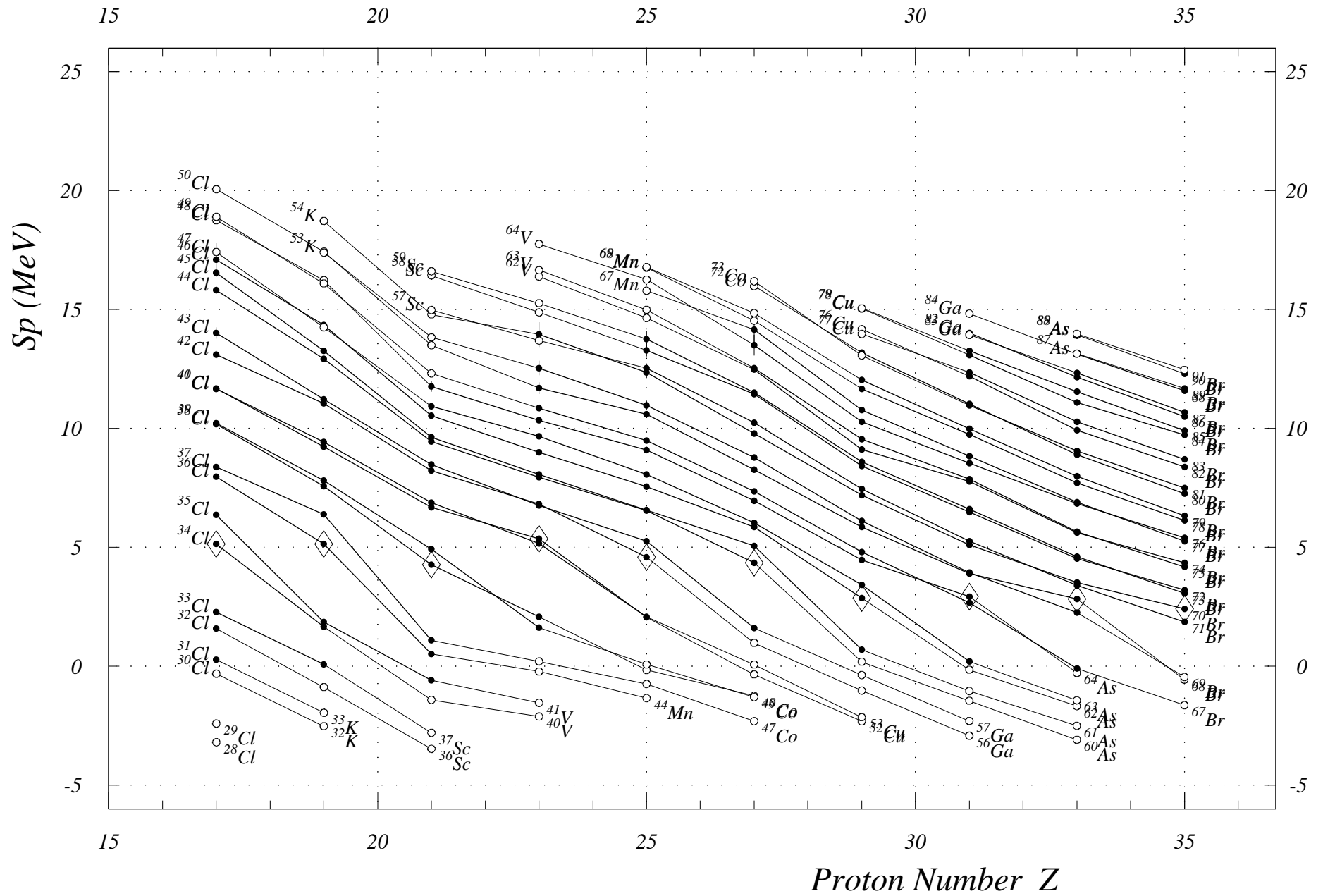
Fig. 11. One-Proton Sep. Energies (odd Z) Z = 17 to 35
