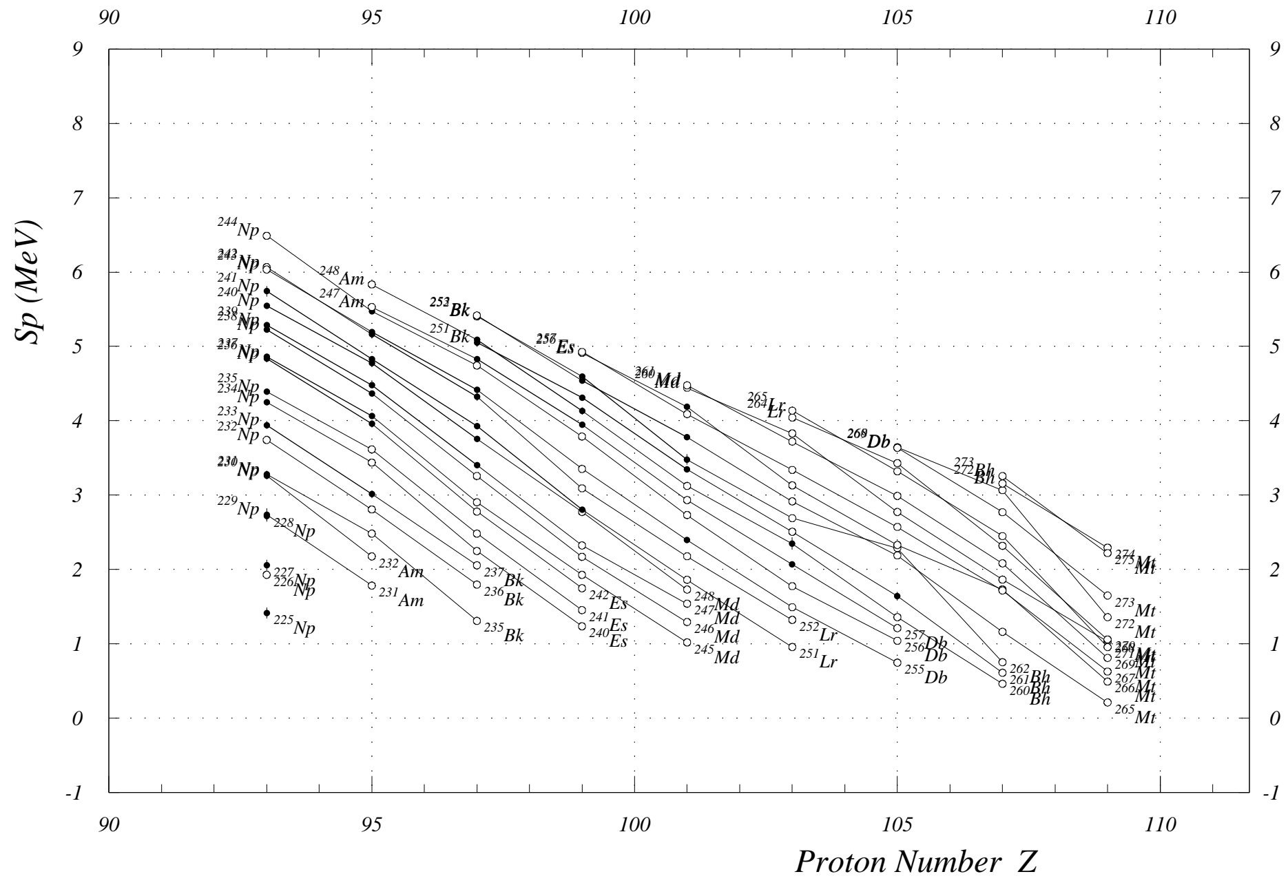
Fig. 16. One-Proton Sep. Energies (odd Z) Z = 92 to 110
