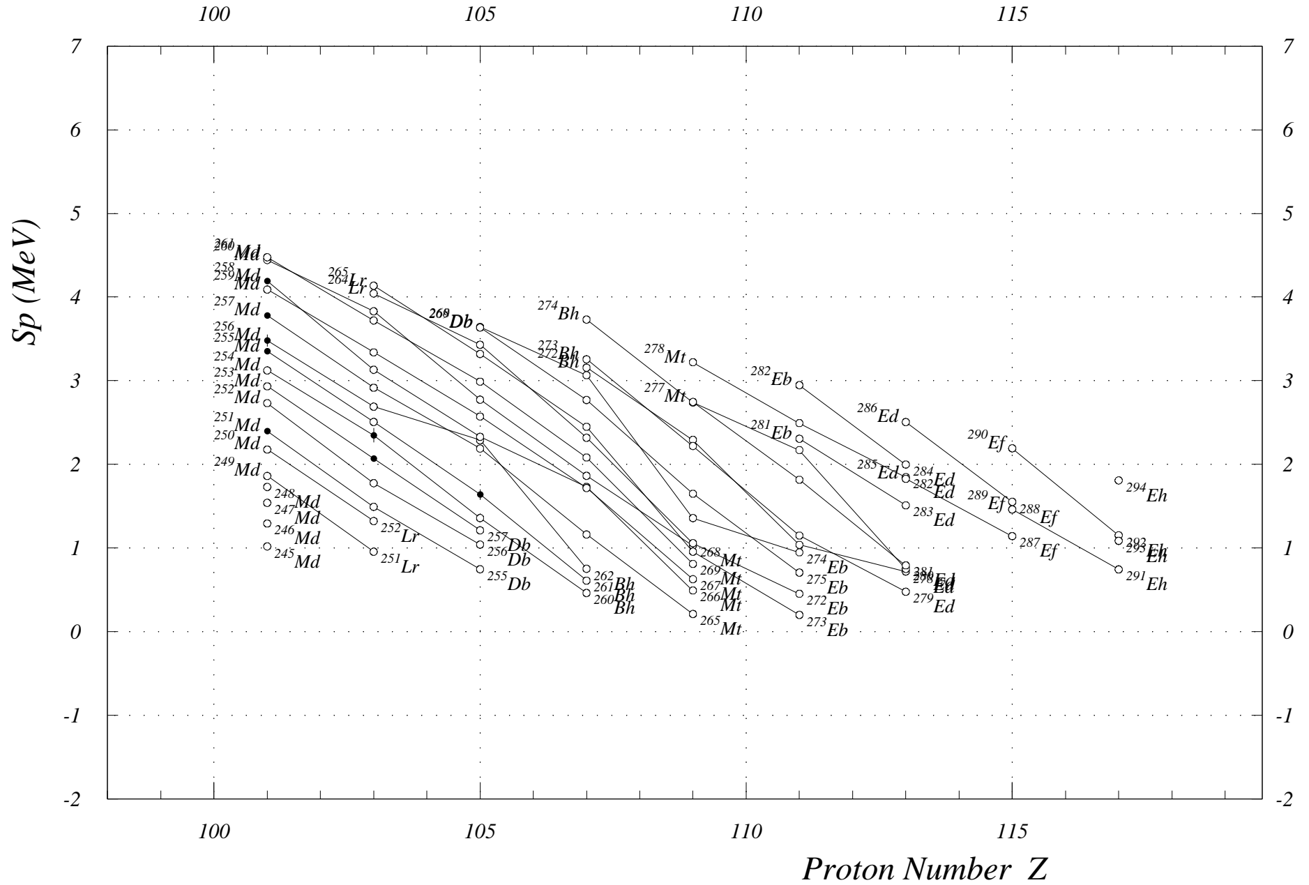
Fig. 17. One-Proton Sep. Energies (odd Z) Z = 100 to 118
