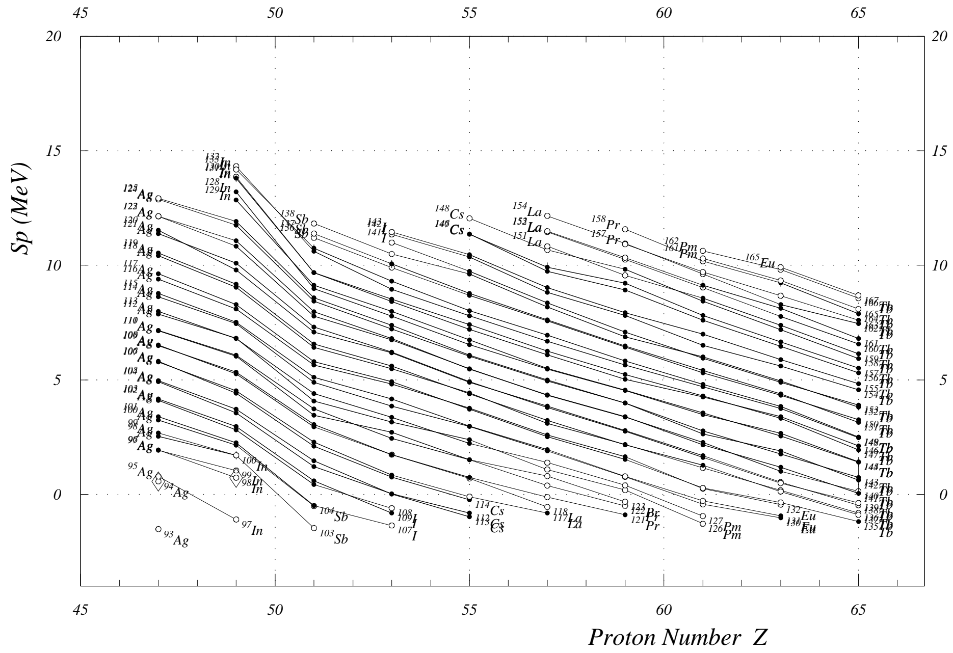
Fig. 13. One-Proton Sep. Energies (odd Z) Z = 47 to 65
