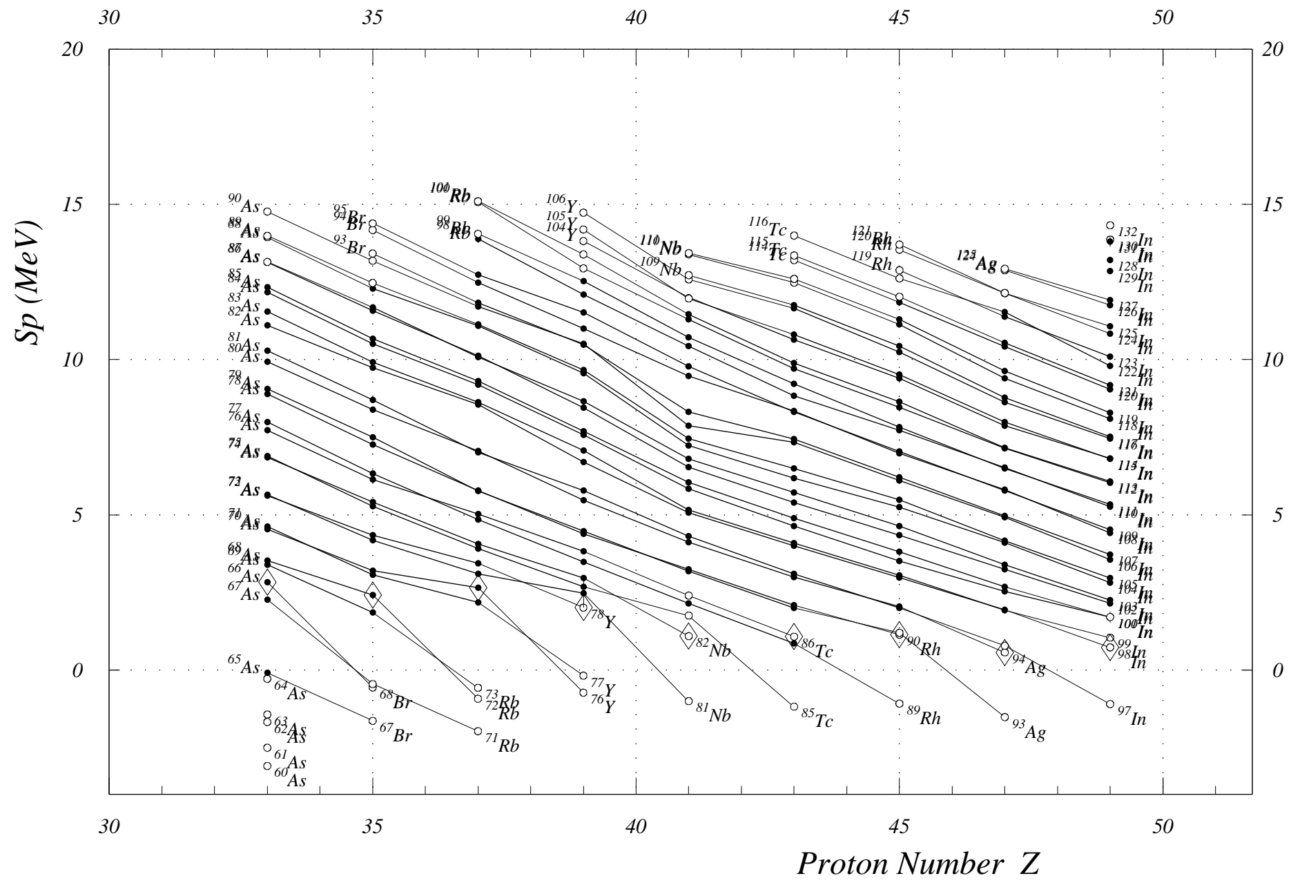
Fig. 12. One-Proton Sep. Energies (odd Z) Z = 32 to 50
