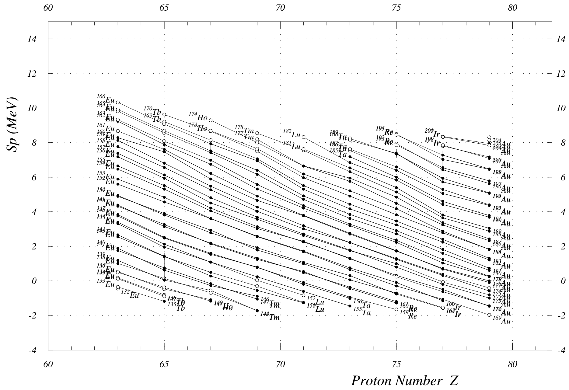
Fig. 14. One-Proton Sep. Energies (odd Z) Z = 62 to 80
