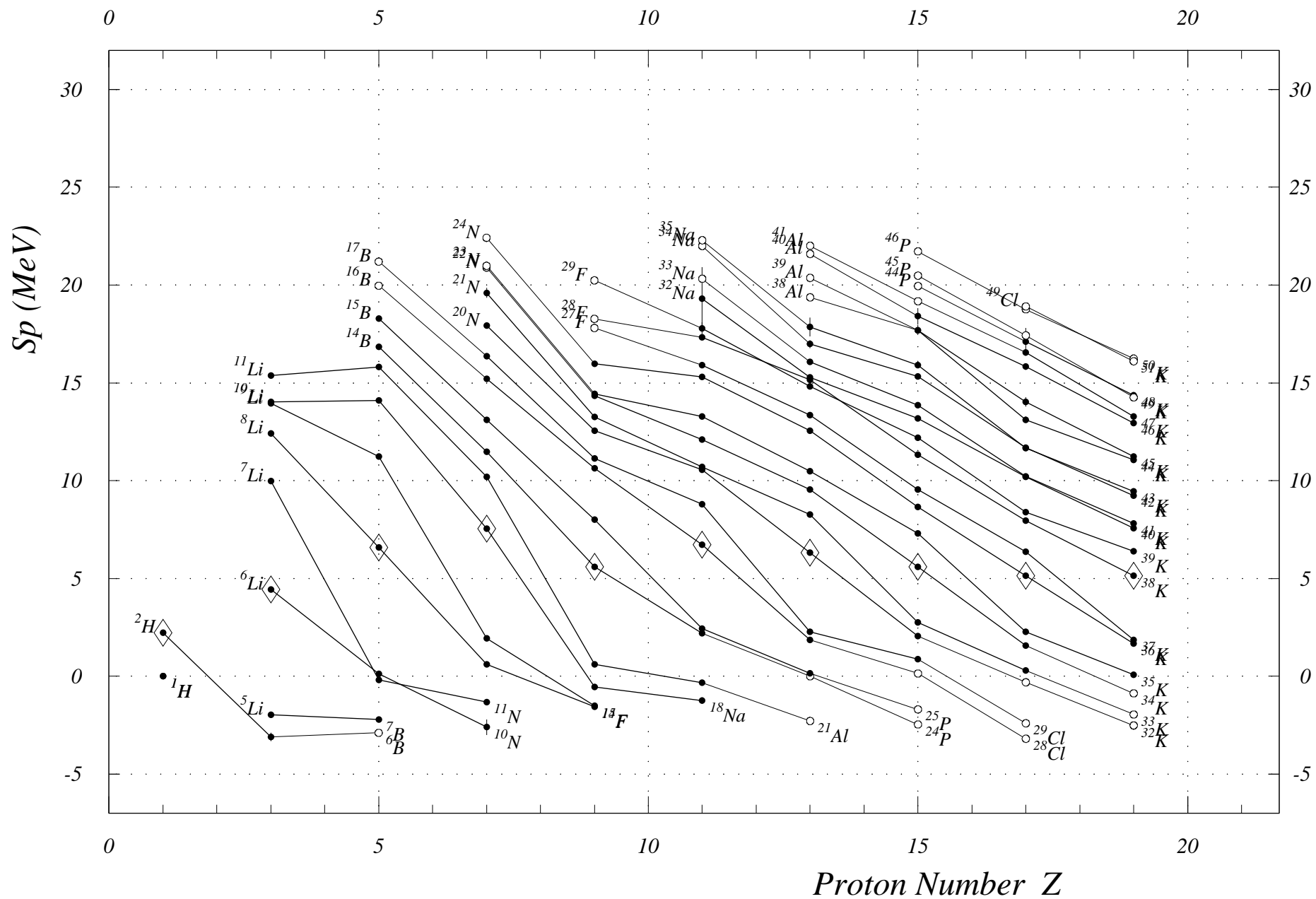
Fig. 10. One-Proton Sep. Energies (odd Z) Z = 0 to 20
