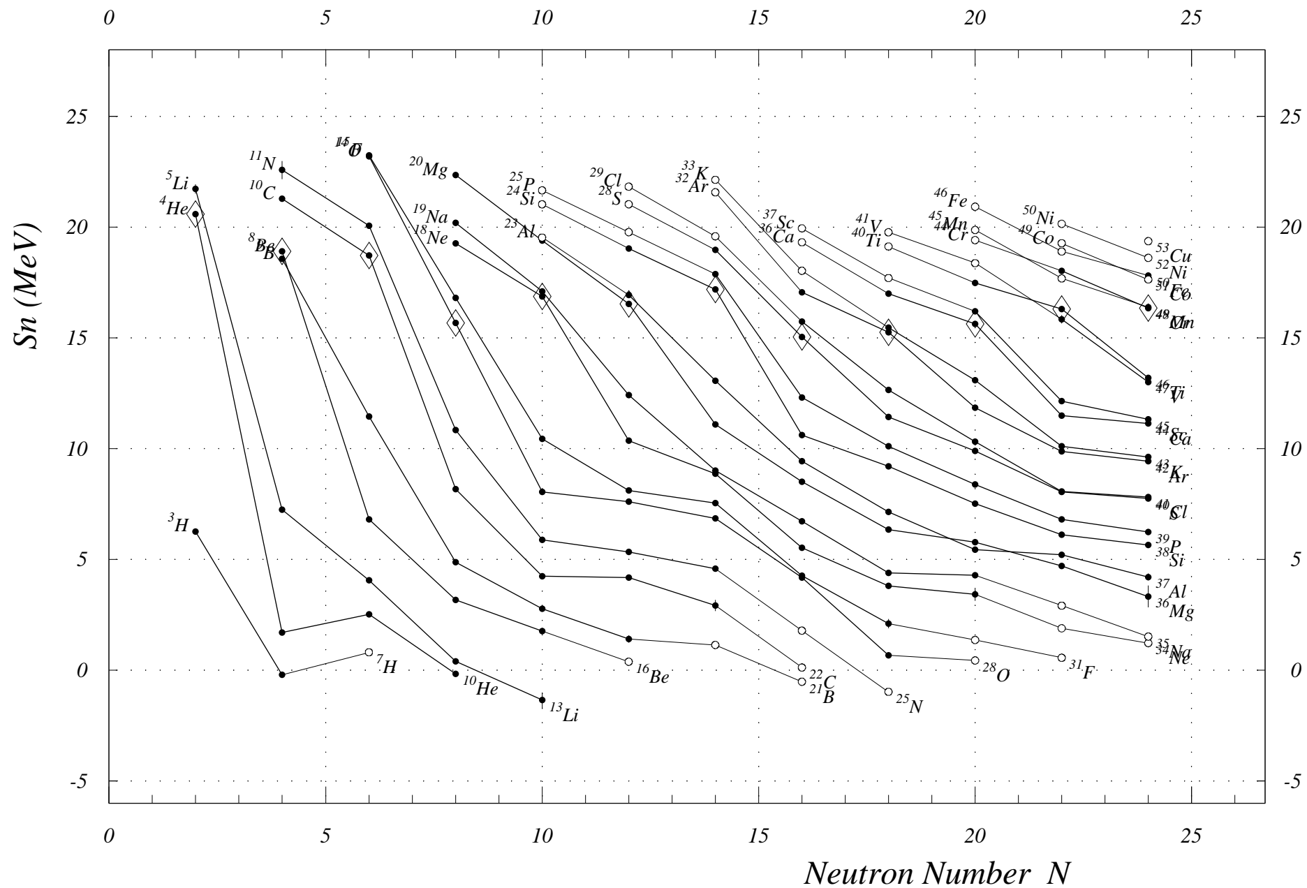
Fig. 1. One-neutron Sep.Energies (even N ) N = 0 to 25
