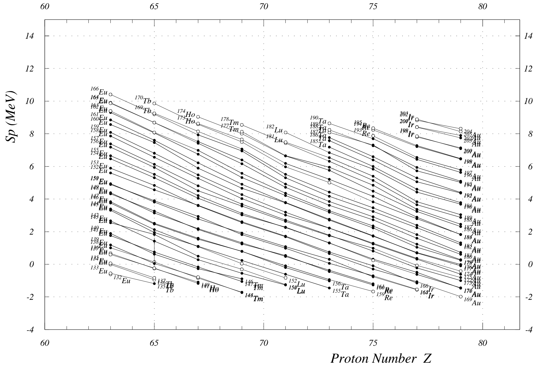
Fig. 14. One-Proton Sep. Energies (odd Z) Z = 62 to 80
