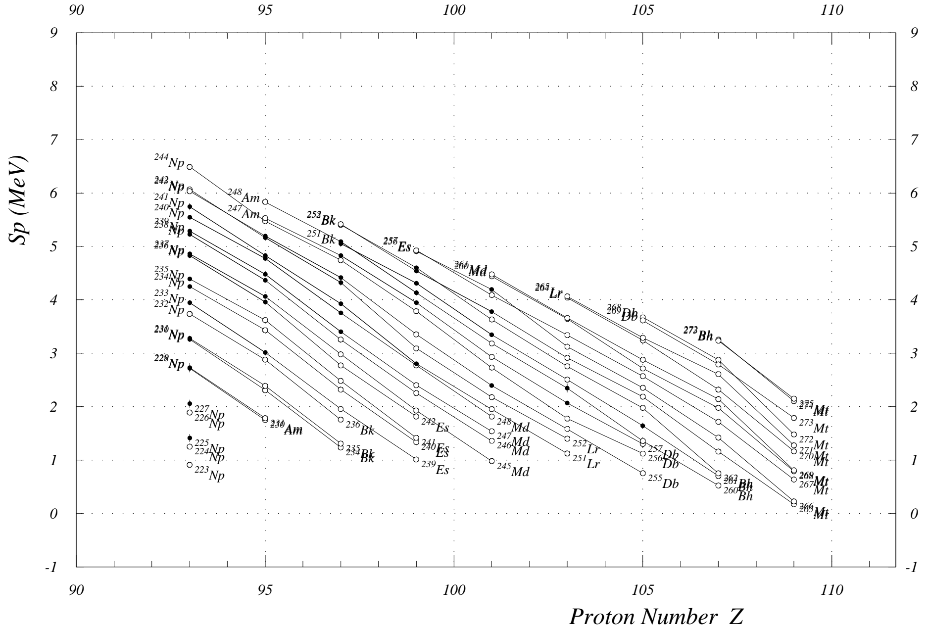
Fig. 16. One-Proton Sep. Energies (odd Z) Z = 92 to 110
