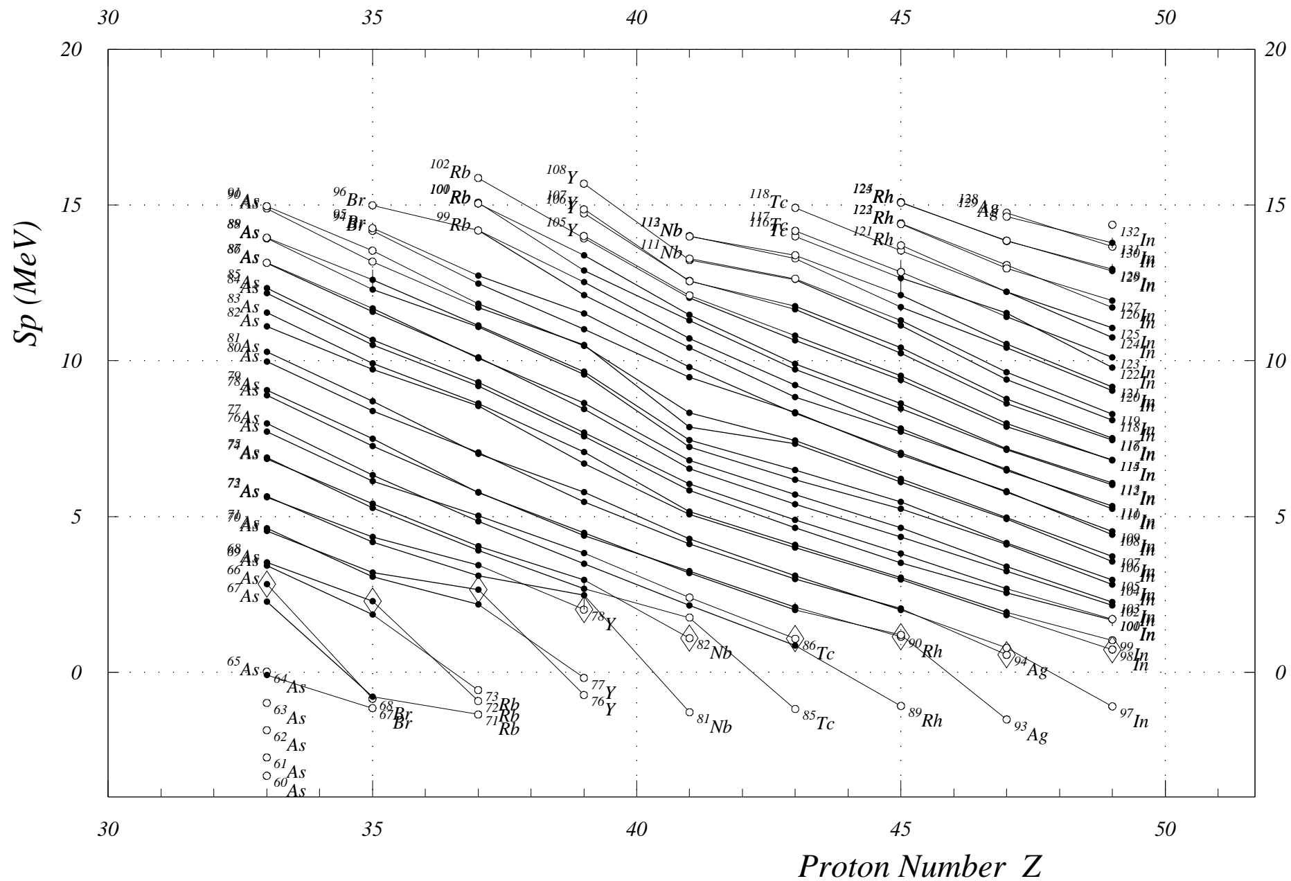
Fig. 12. One-Proton Sep. Energies (odd Z) Z = 32 to 50
