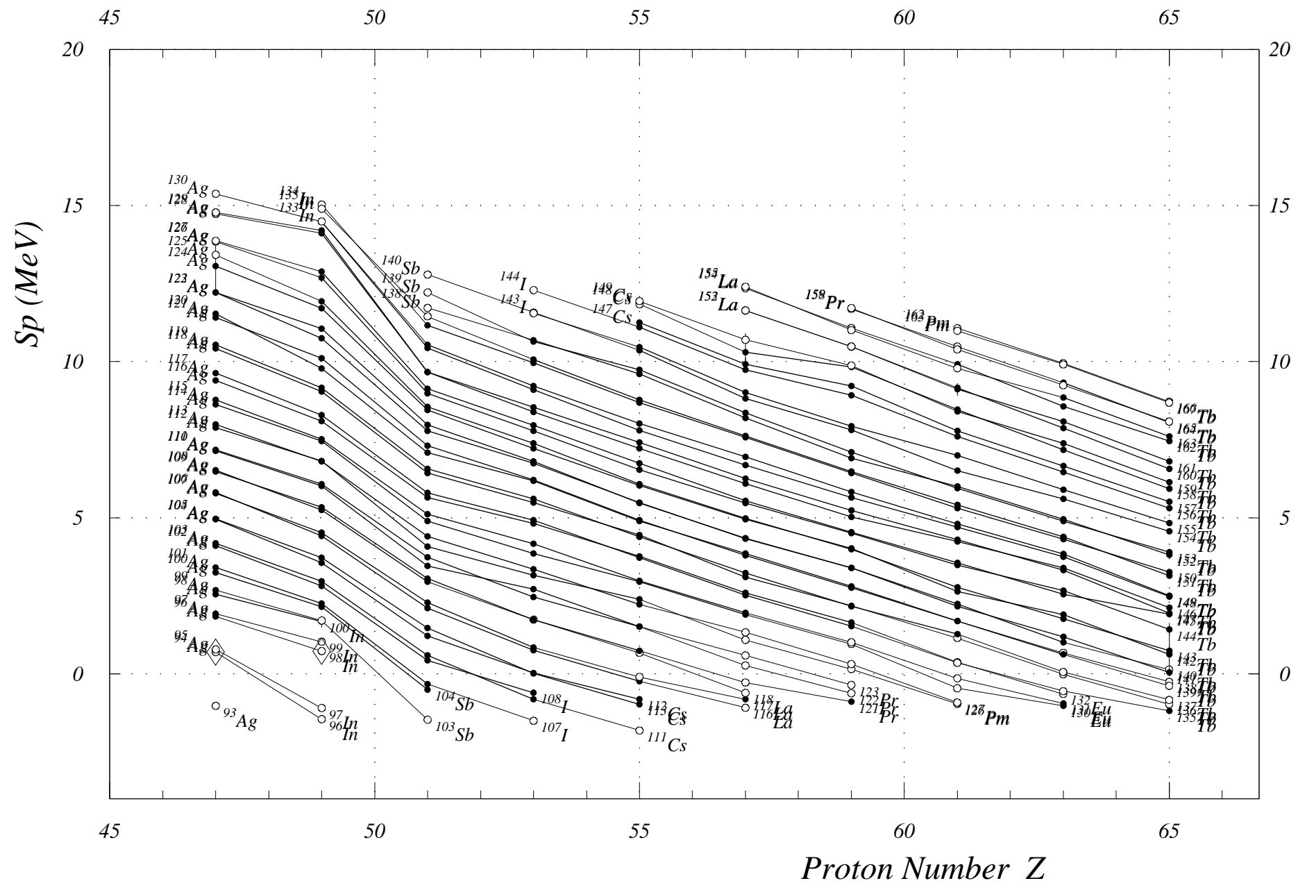
Fig. 4. One-Proton Sep. Energies (odd Z) Z = 47 to 65
