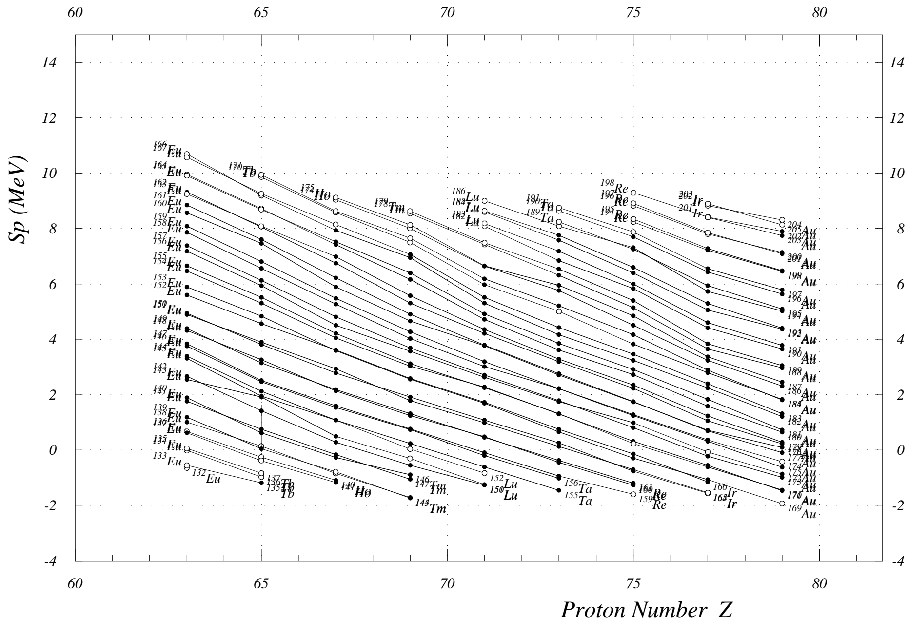
Fig. 5. One-Proton Sep. Energies (odd Z) Z = 62 to 80
