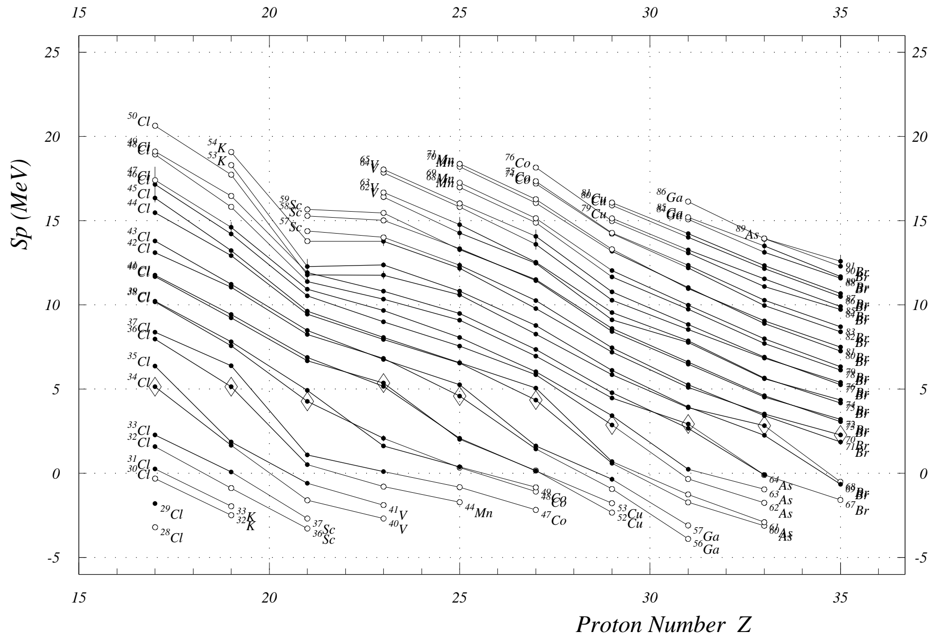
Fig. 2. One-Proton Sep. Energies (odd Z) Z = 17 to 35
