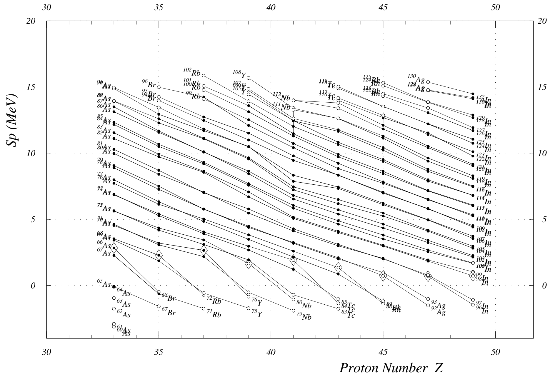
Fig. 3. One-Proton Sep. Energies (odd Z) Z = 32 to 50
