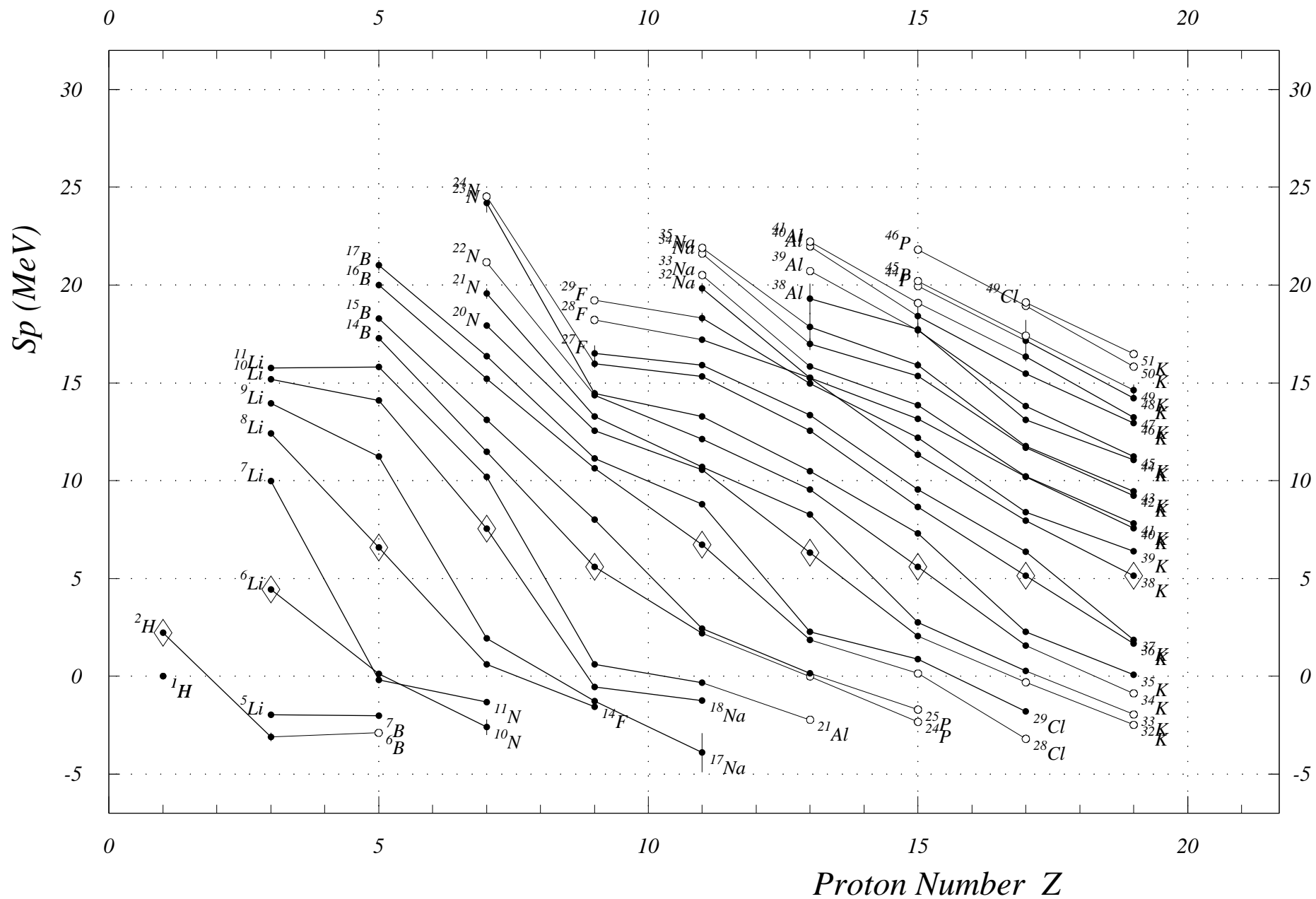
Fig. 1. One-Proton Sep. Energies (odd Z) Z = 0 to 20
