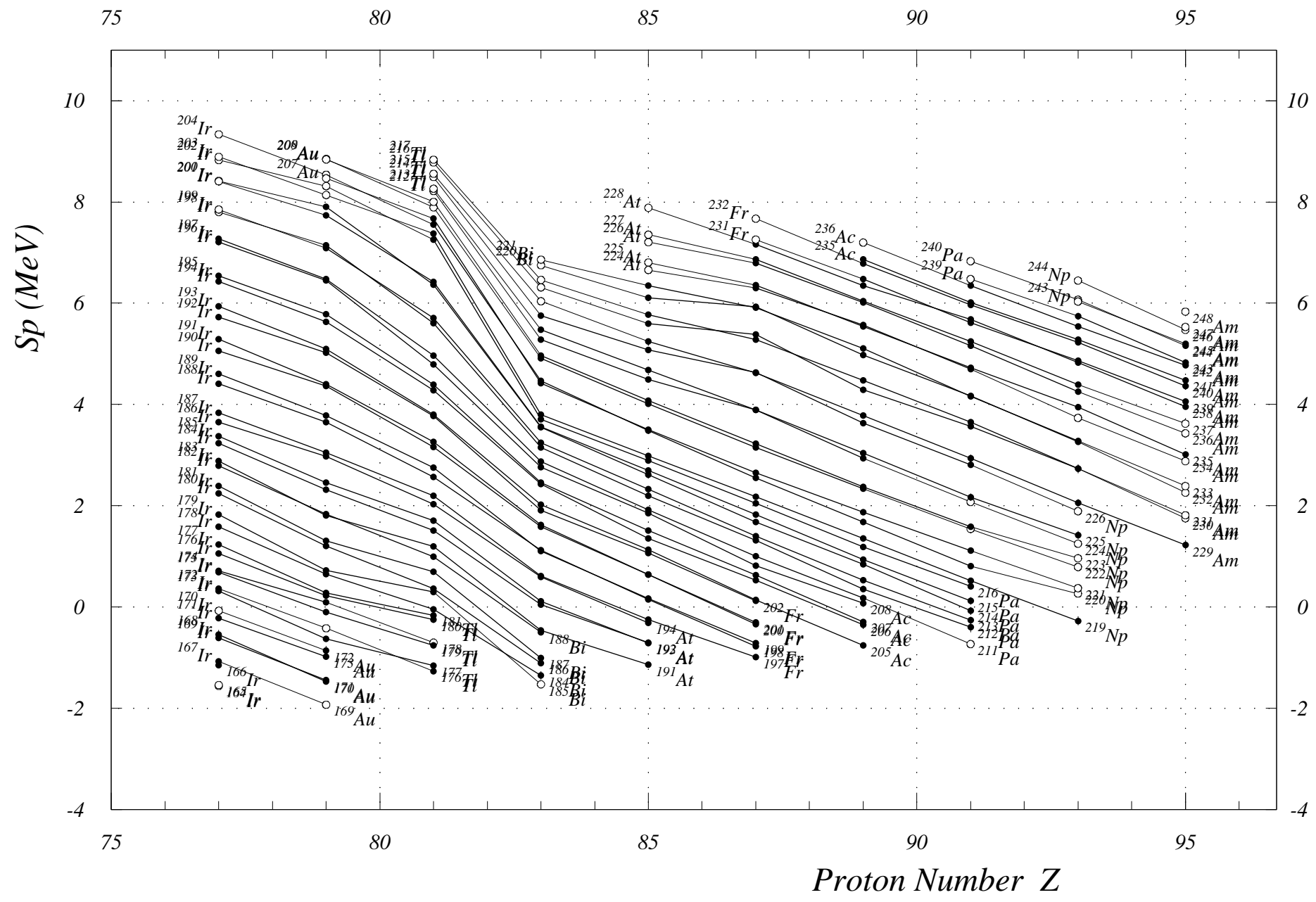
Fig. 6. One-Proton Sep. Energies (odd Z) Z = 77 to 95
