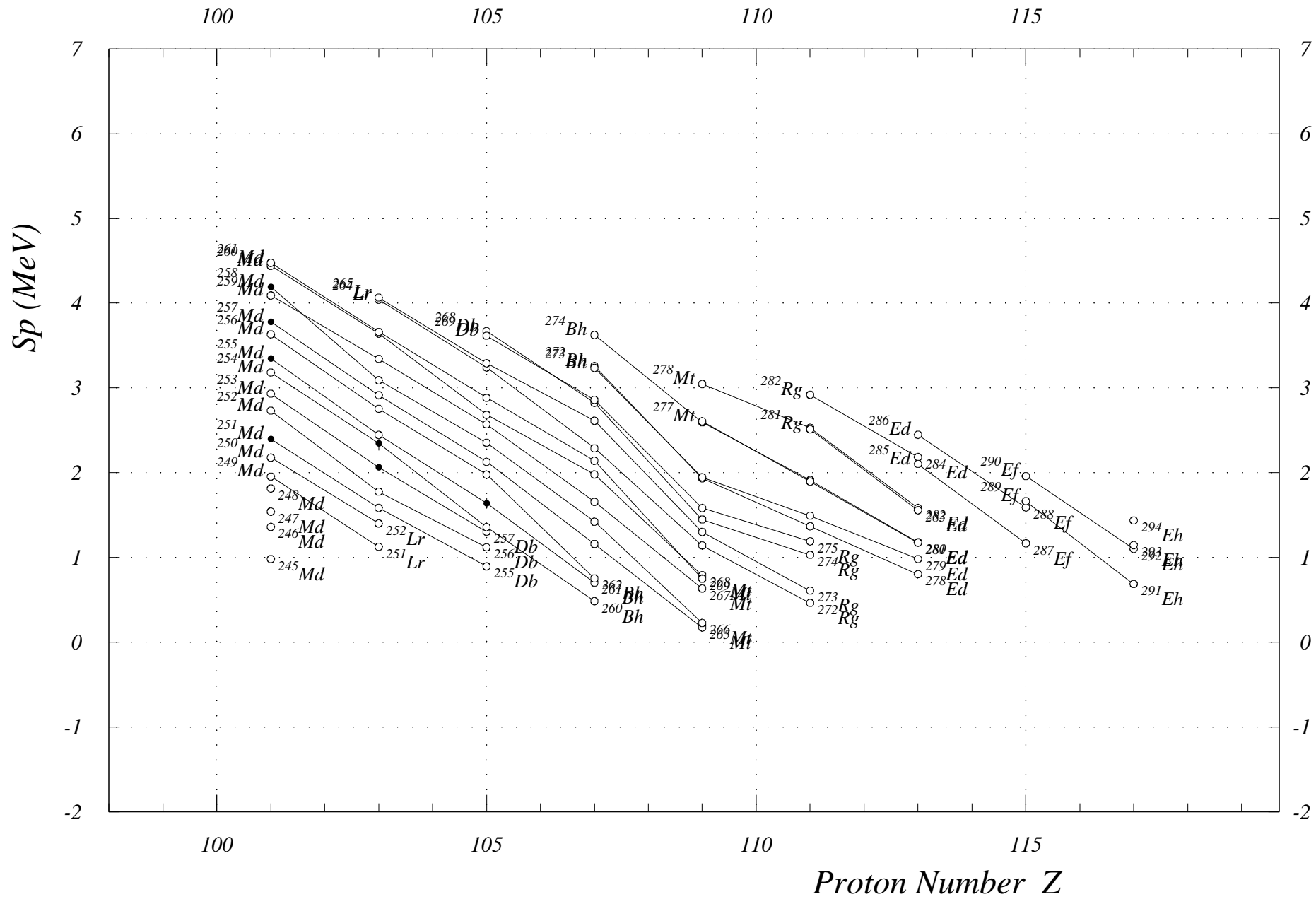
Fig. 8. One-Proton Sep. Energies (odd Z) Z = 100 to 118
