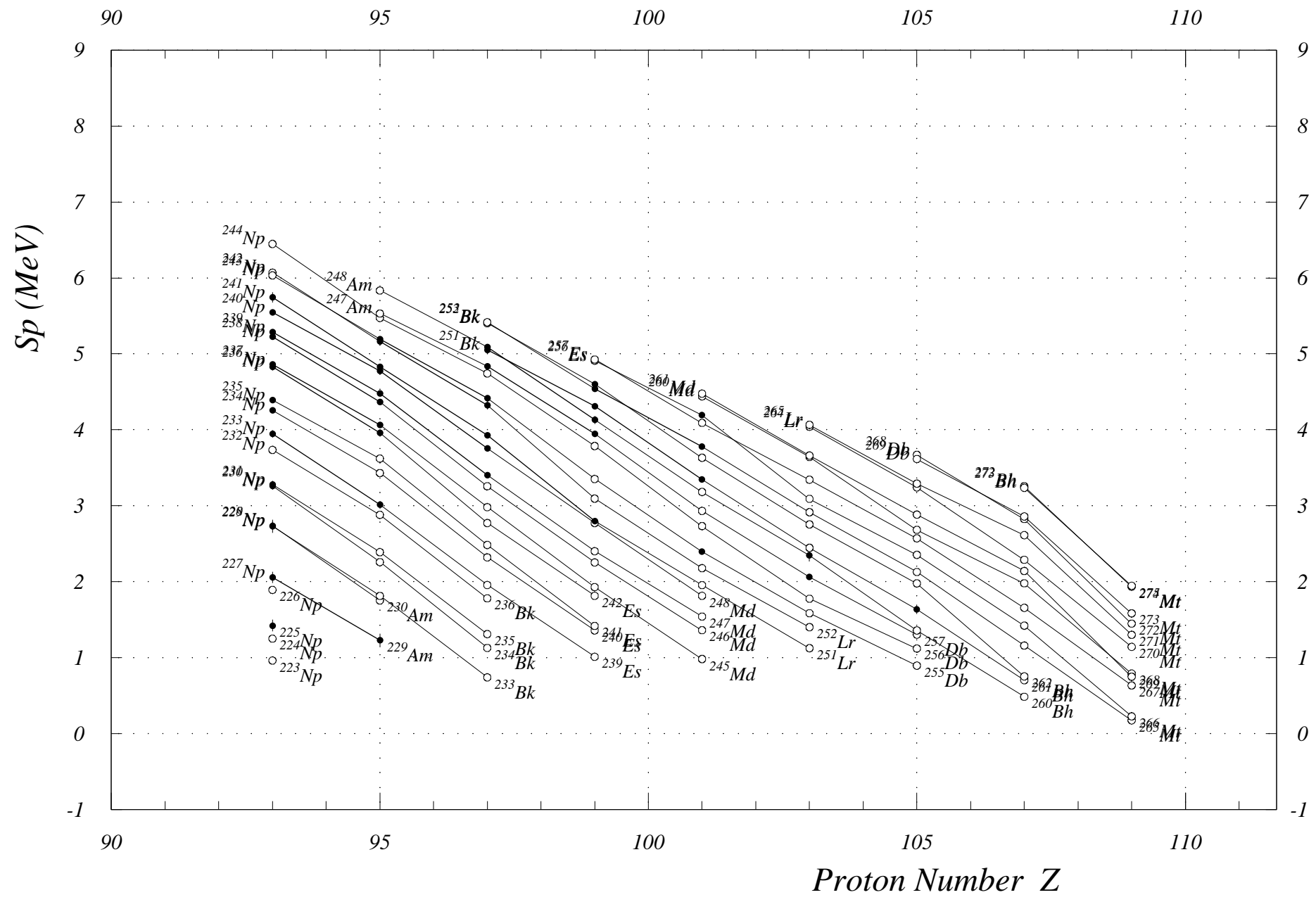
Fig. 7. One-Proton Sep. Energies (odd Z) Z = 92 to 110
