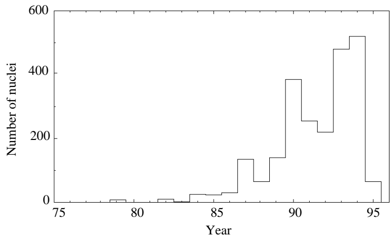
Figure 1. ENSDF status (total number of nuclei = 2347).
